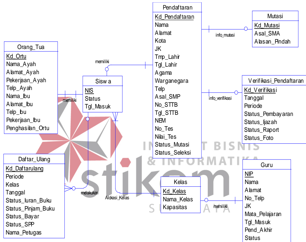
Gambar 4.14 CDM
