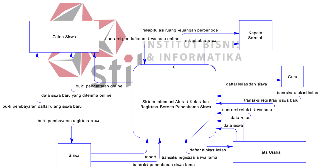
Gambar 4.6 Context Diagram
