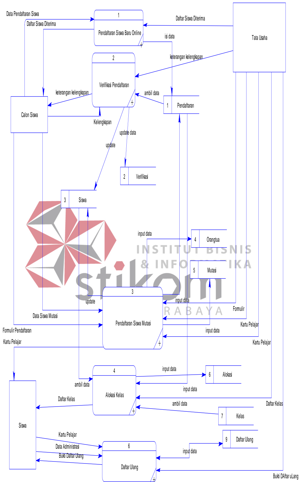
Gambar 4.8 DFD Level 0
