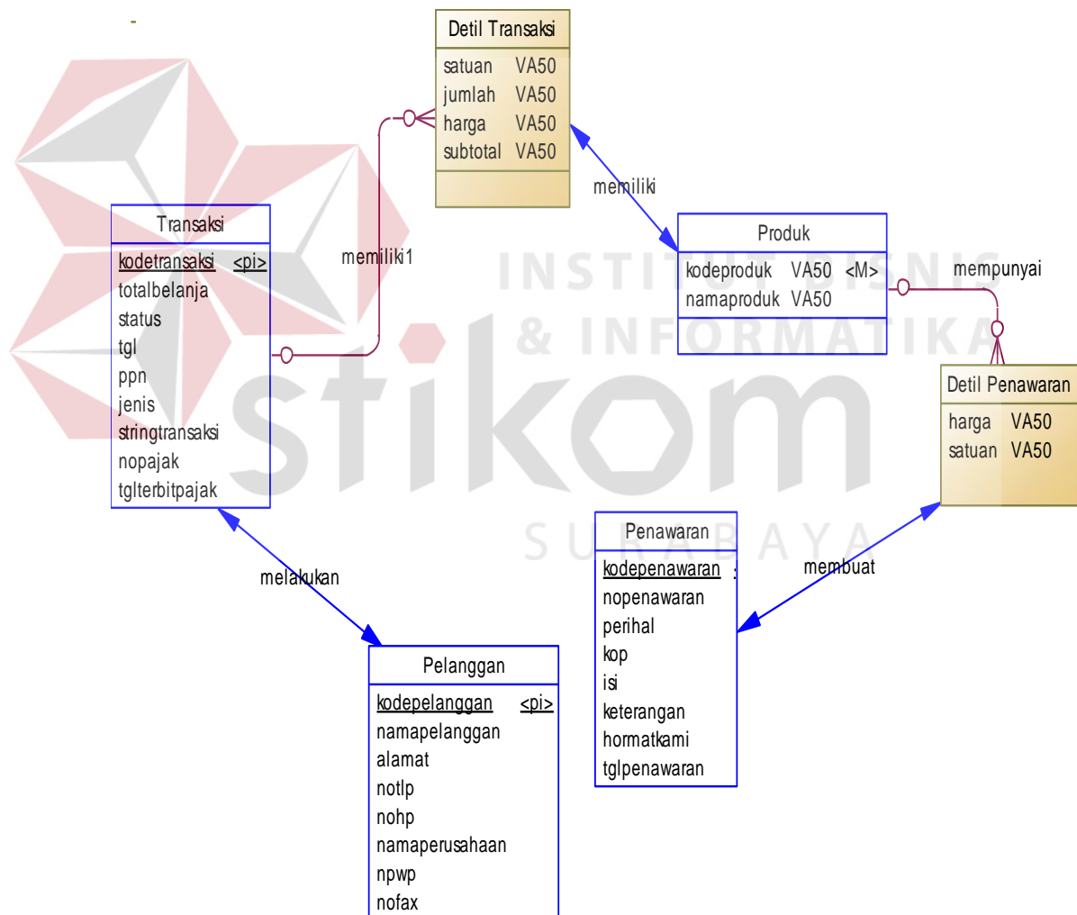
Gambar 4.16 Conceptual Data Model
