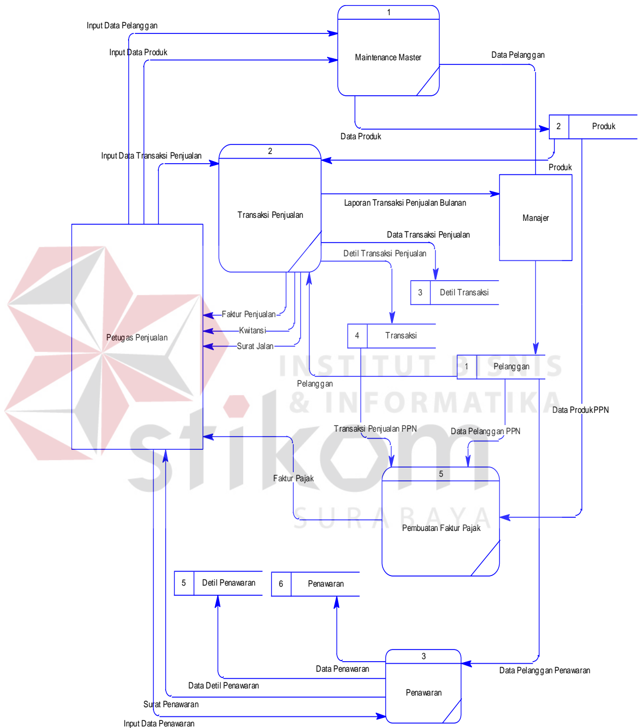
Gambar 4.11 Data Flow Diagram Level 0
