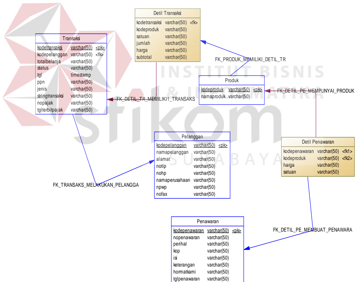
Gambar 4.17 Physical Data Model
