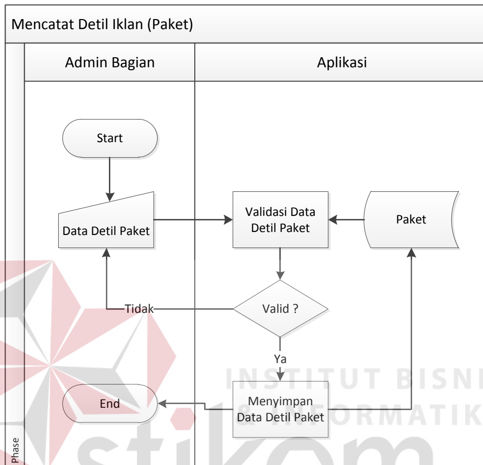
Gambar 4.5 System Flow Detil Iklan (Paket)
