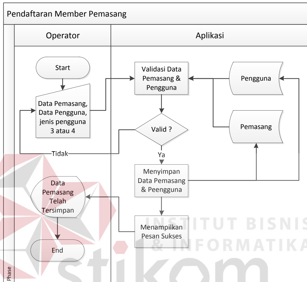
Gambar 4.6 System Flow Mencatat Member Pemasang
