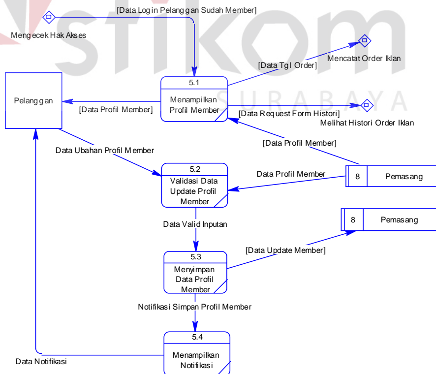
Gambar 4.18 DFD Level 1 Mengelola Profil Member
