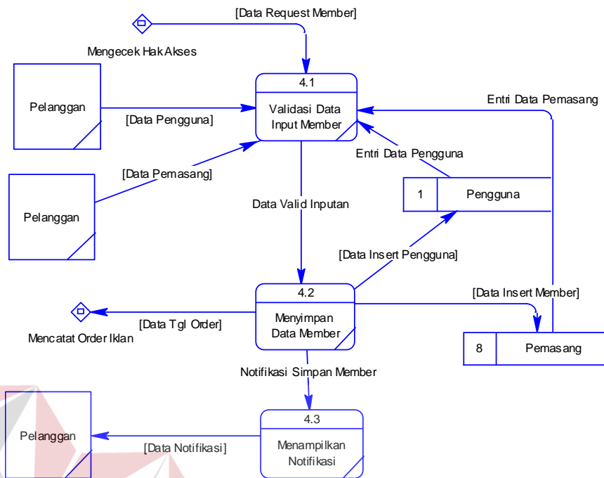
Gambar 4.17 DFD Level 1 Mencatat Pendaftaran Member
