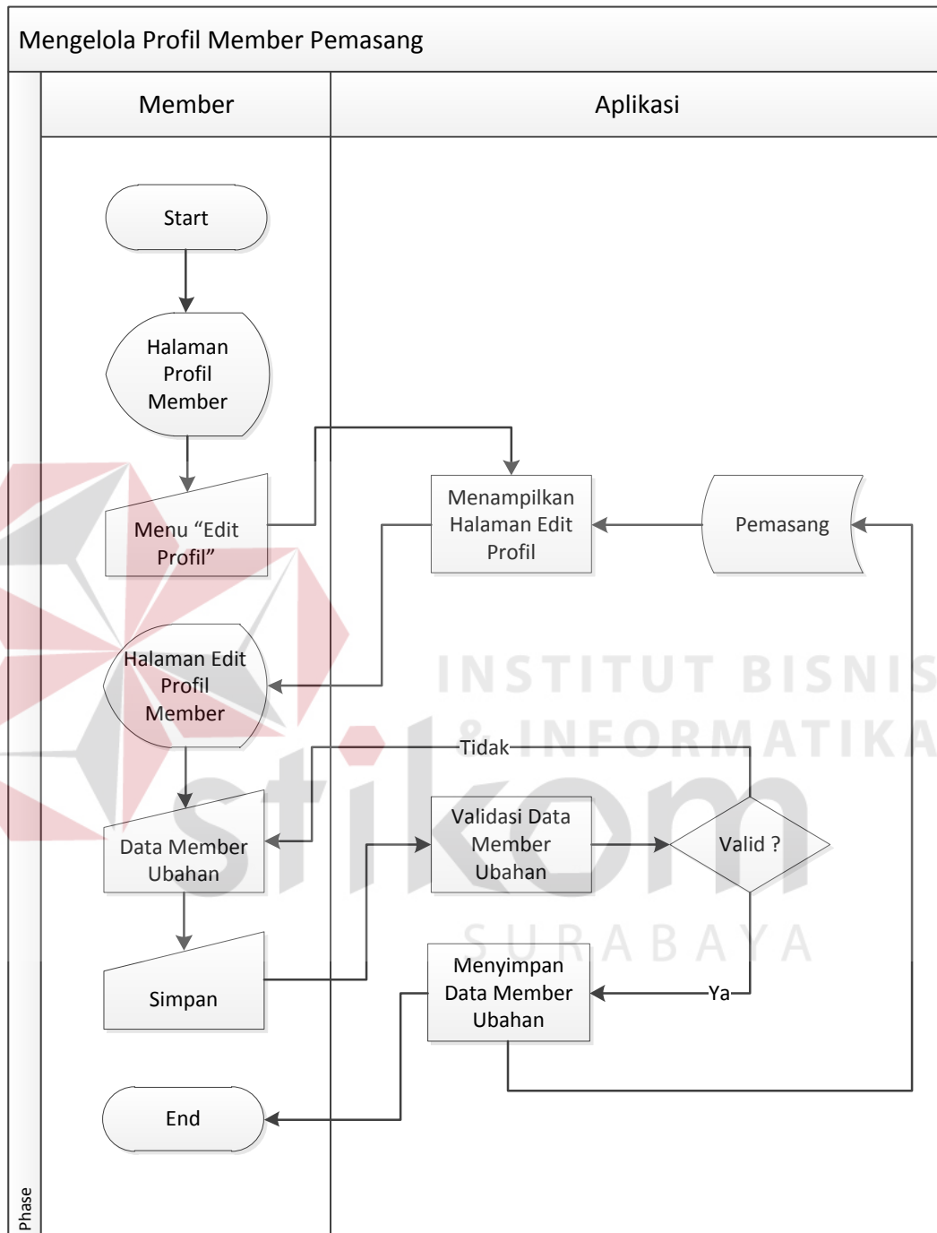
Gambar 4.7 System Flow Profil Member Pemasng
