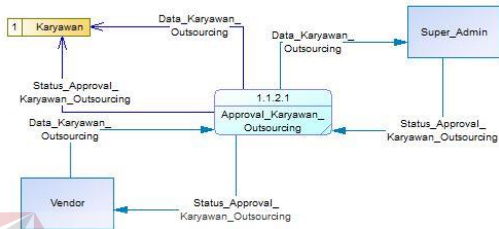
Gambar 4.16 Data Flow Diagram Level 2 Registrasi Karyawan Outsourcing
