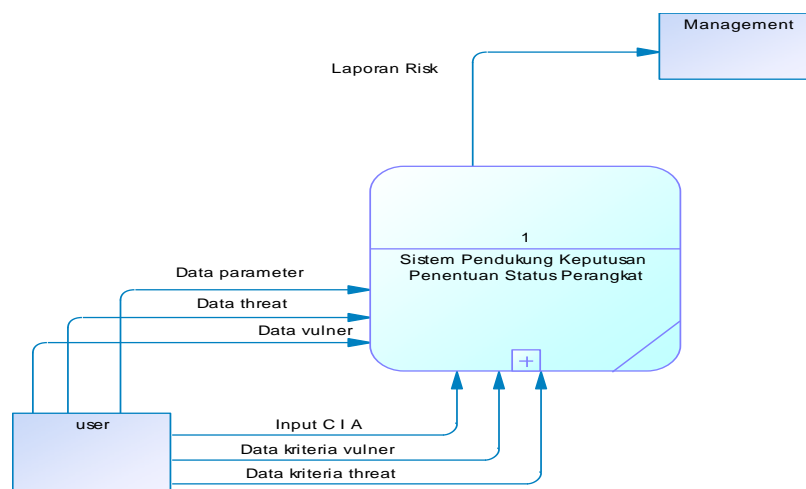
Gambar 4.2 Context Diagram
