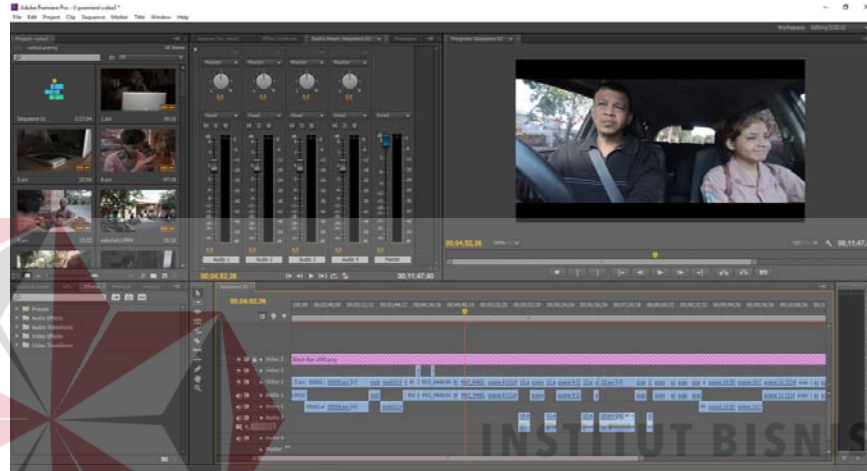
Gambar 4.20 Proses Export/Rendering
