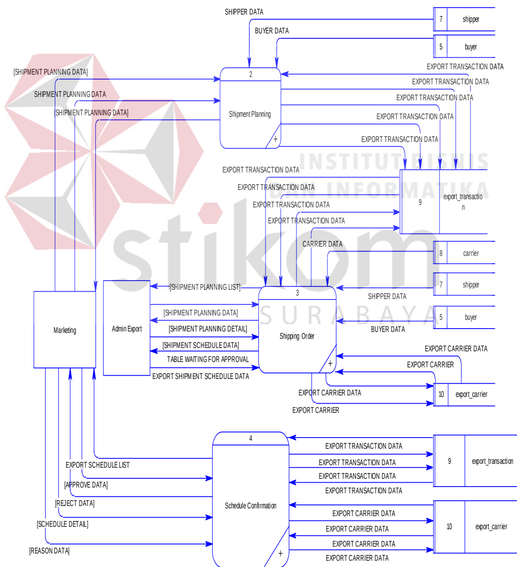
Gambar 0.19 Data flow diagram level 0 transaction
