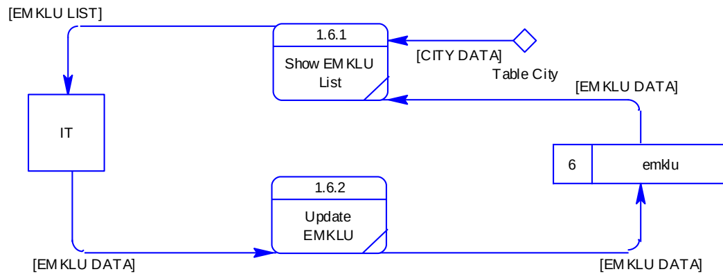
Gambar 0.29 Data flow diagram level 2 manage master data EMKLU
