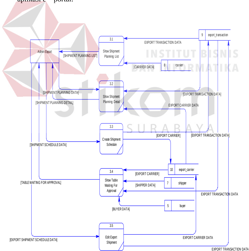
Gambar 0.22 Data flow diagram level 1 shipping order
