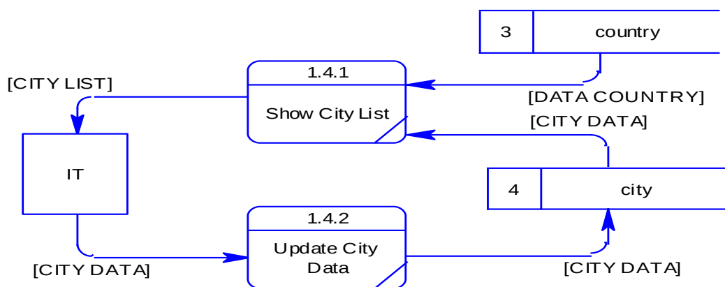
Gambar 0.27 Data flow diagram level 2 manage master data city
