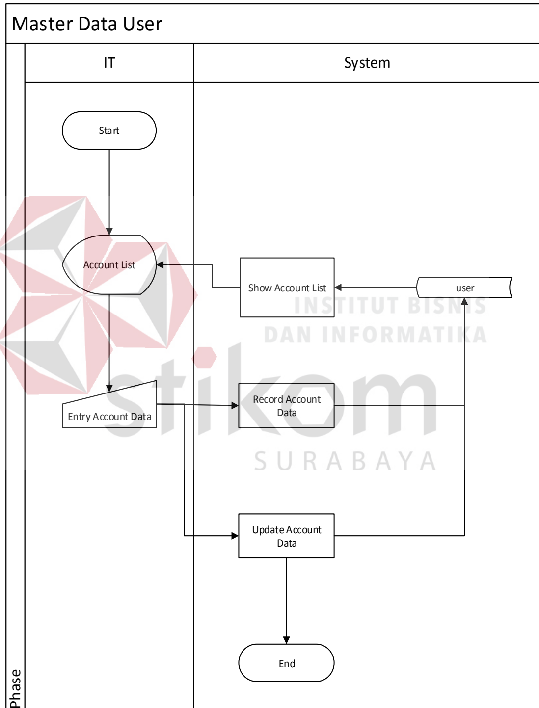
Gambar 0.5 System flow data master user
