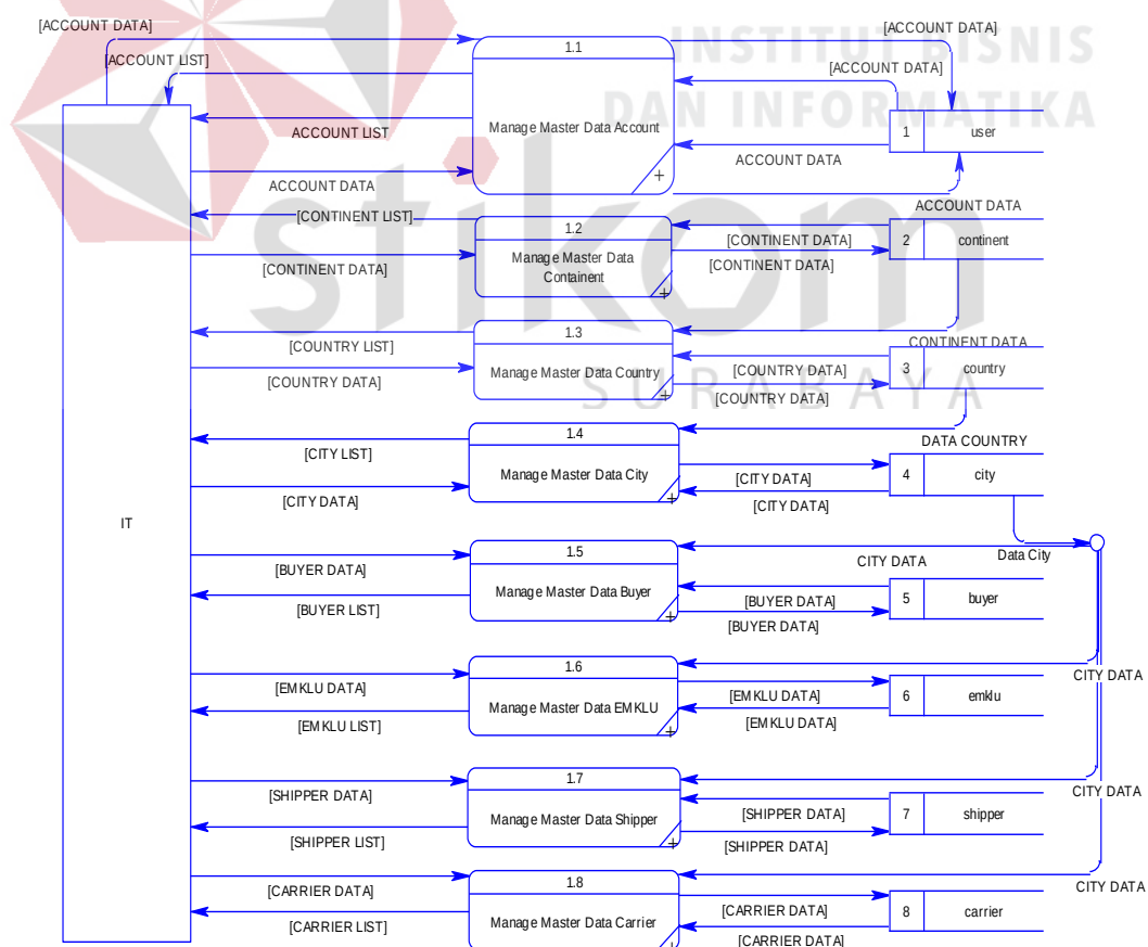
Gambar 0.20 Data flow diagram level 1 manage master data
