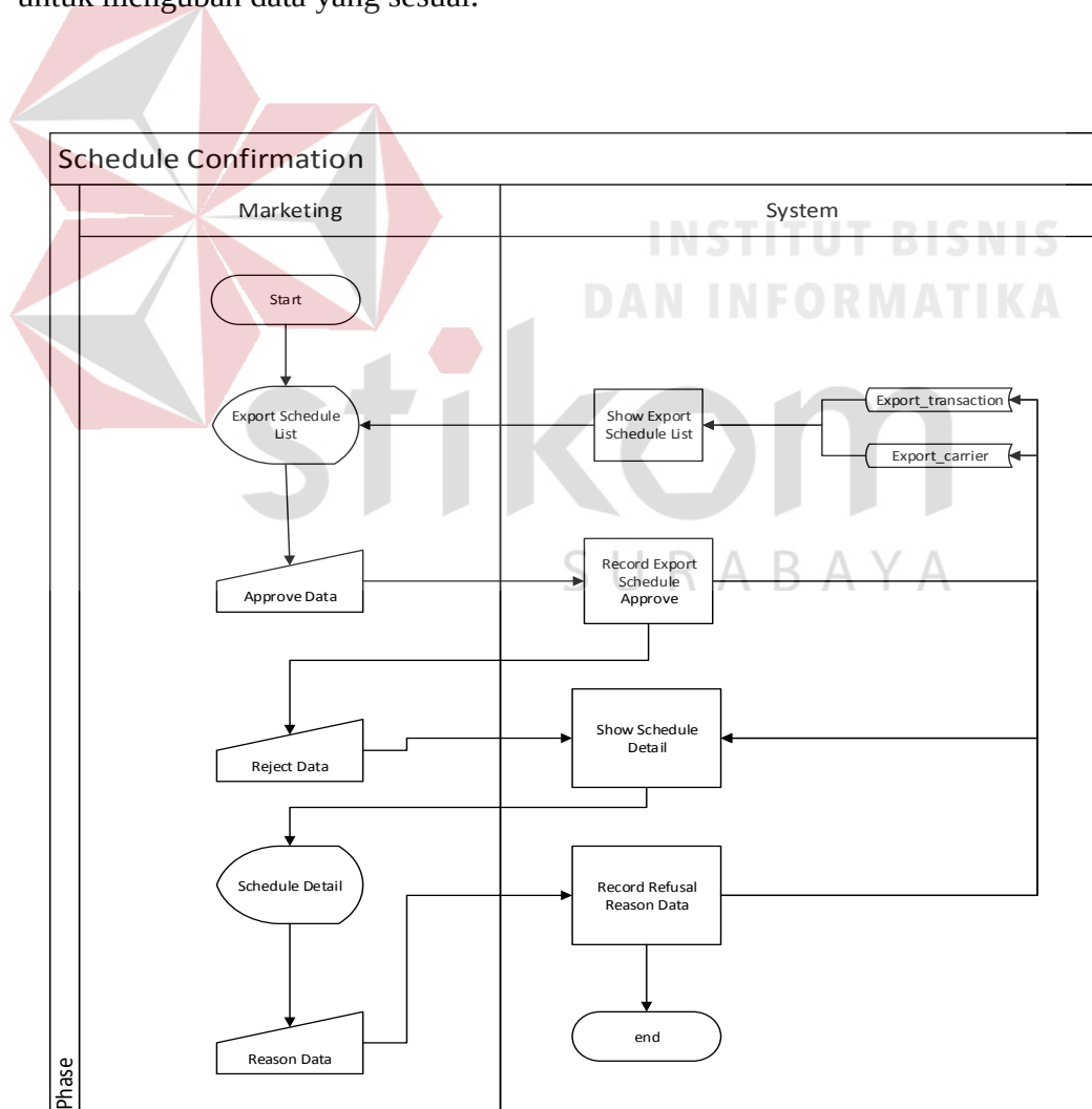
Gambar 0.15 System flow schedule confirmation
