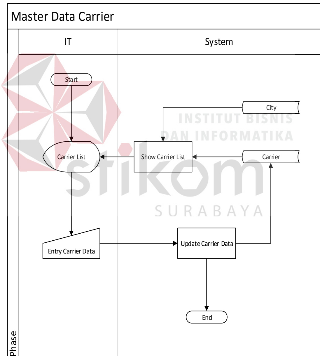
Gambar 0.12 System flow data master carrier
