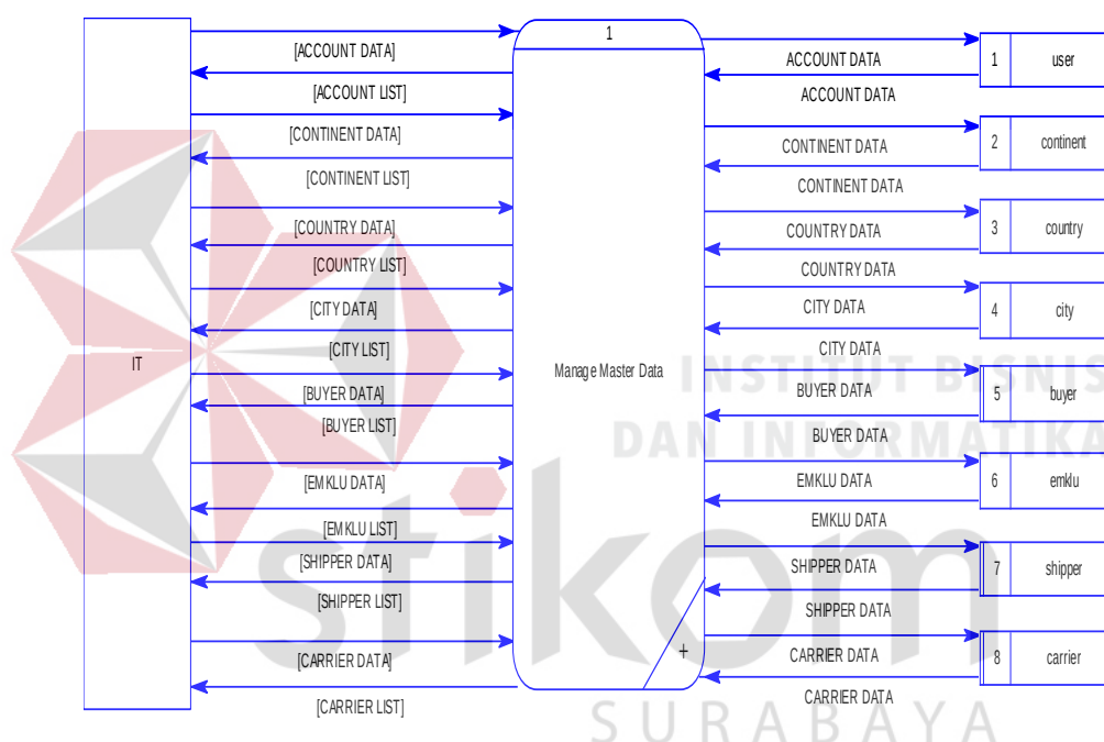
Gambar 0.18 Data flow diagram level 0 manage data master
