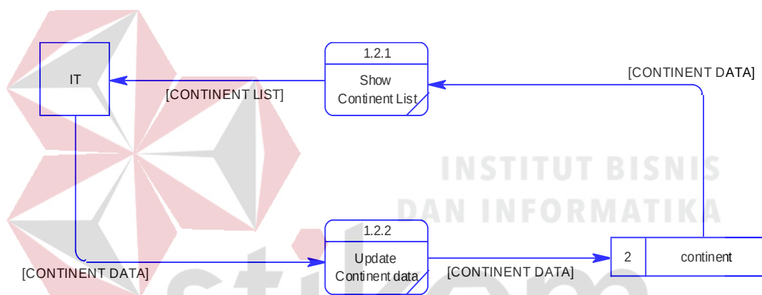
Gambar 0.25 Data flow diagram level 2 manage master data continent
