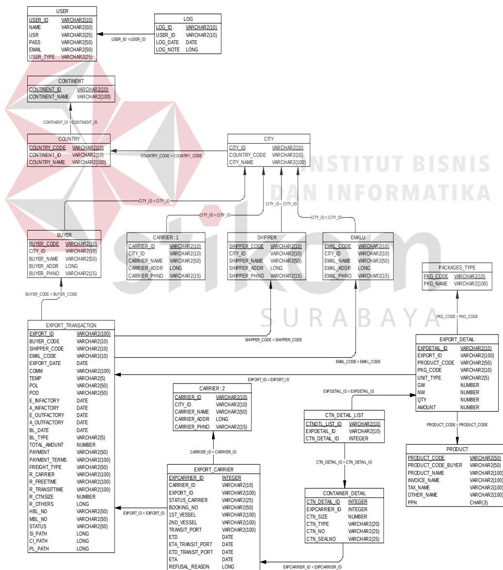
Gambar 0.33 Physical Data Model (PDM)
