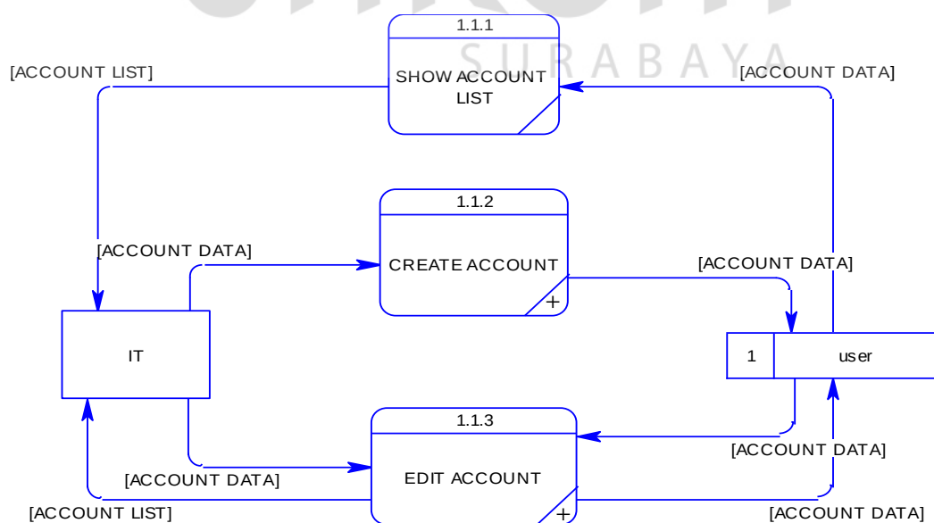
Gambar 0.24 data flow diagram level 2 manage master data account
