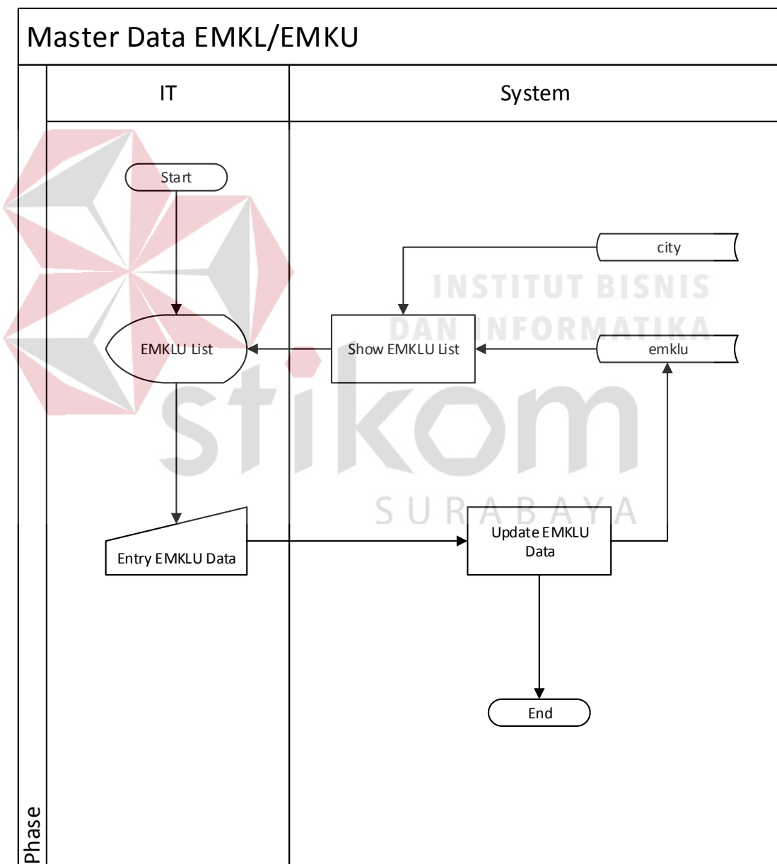
Gambar 0.10 System flow data master EMKLatau EMKU
