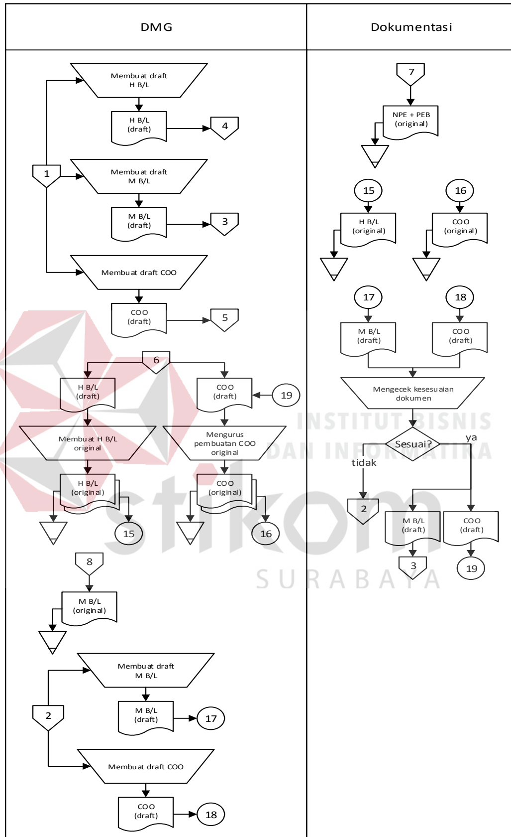
Gambar 0.3 Document Flow Export
