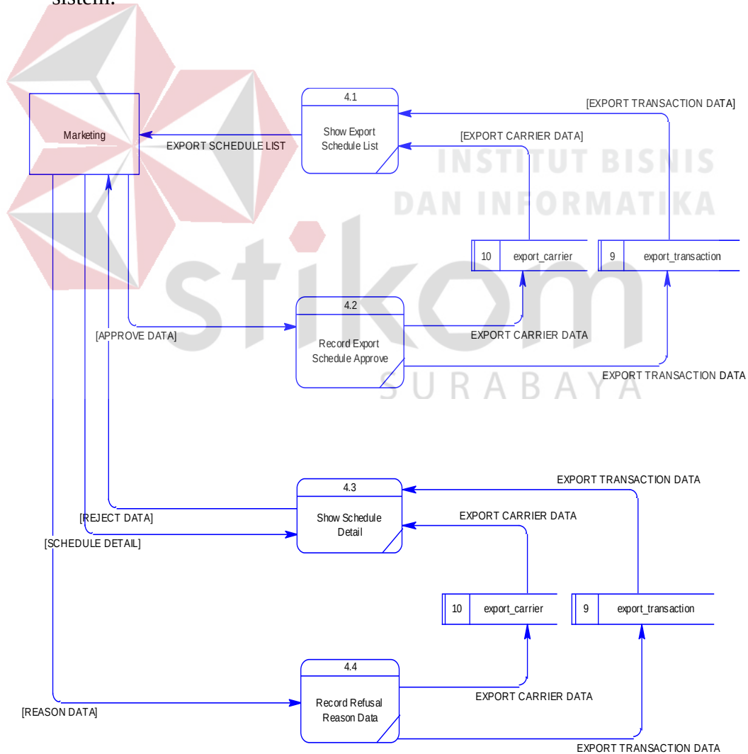
Gambar 0.23 Data flow diagram level 1 confirmation schedule
