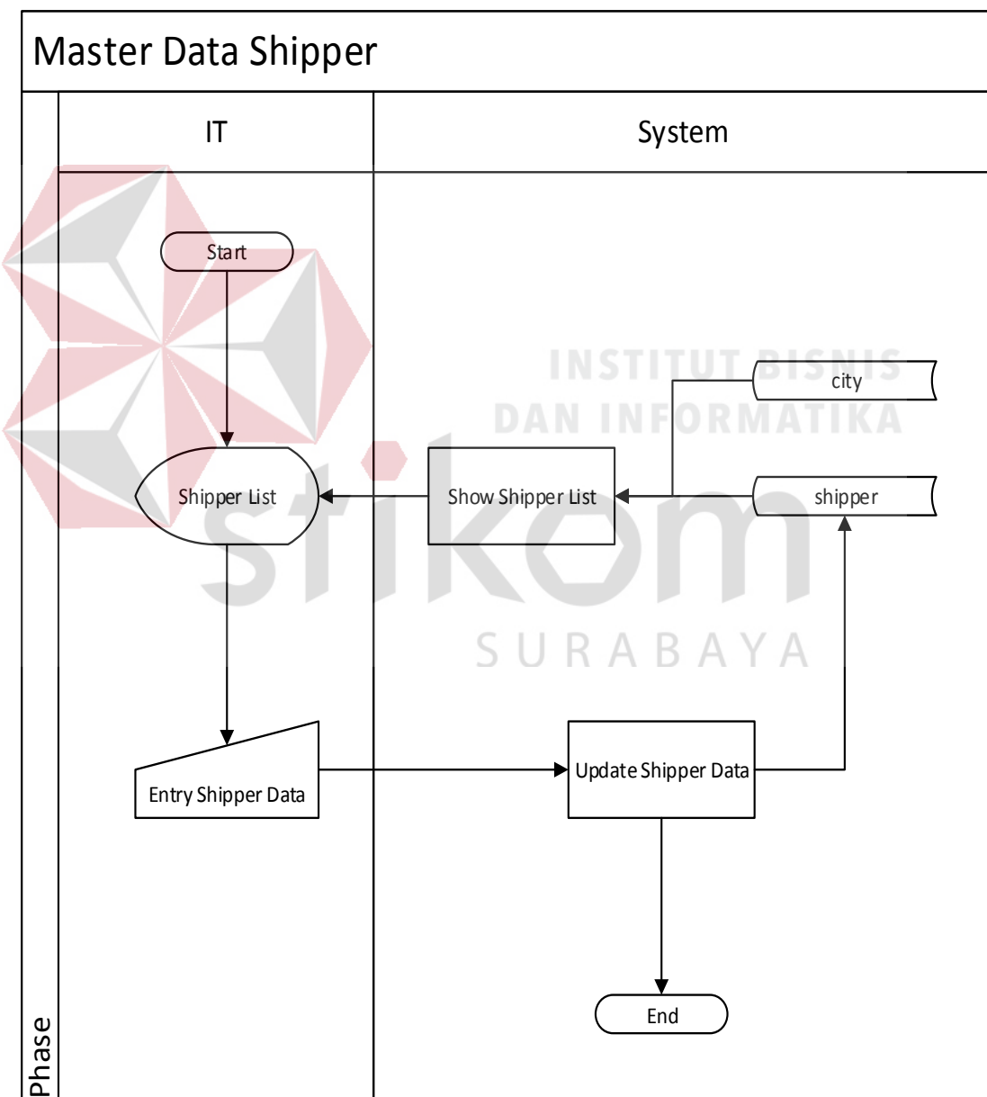
Gambar 0.11 System flow data master shipper
