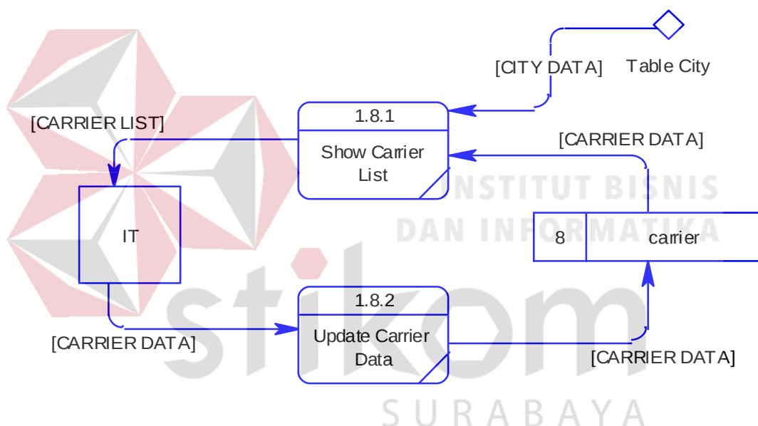
Gambar 0.31 Data flow diagram level 2 manage master data carrier
