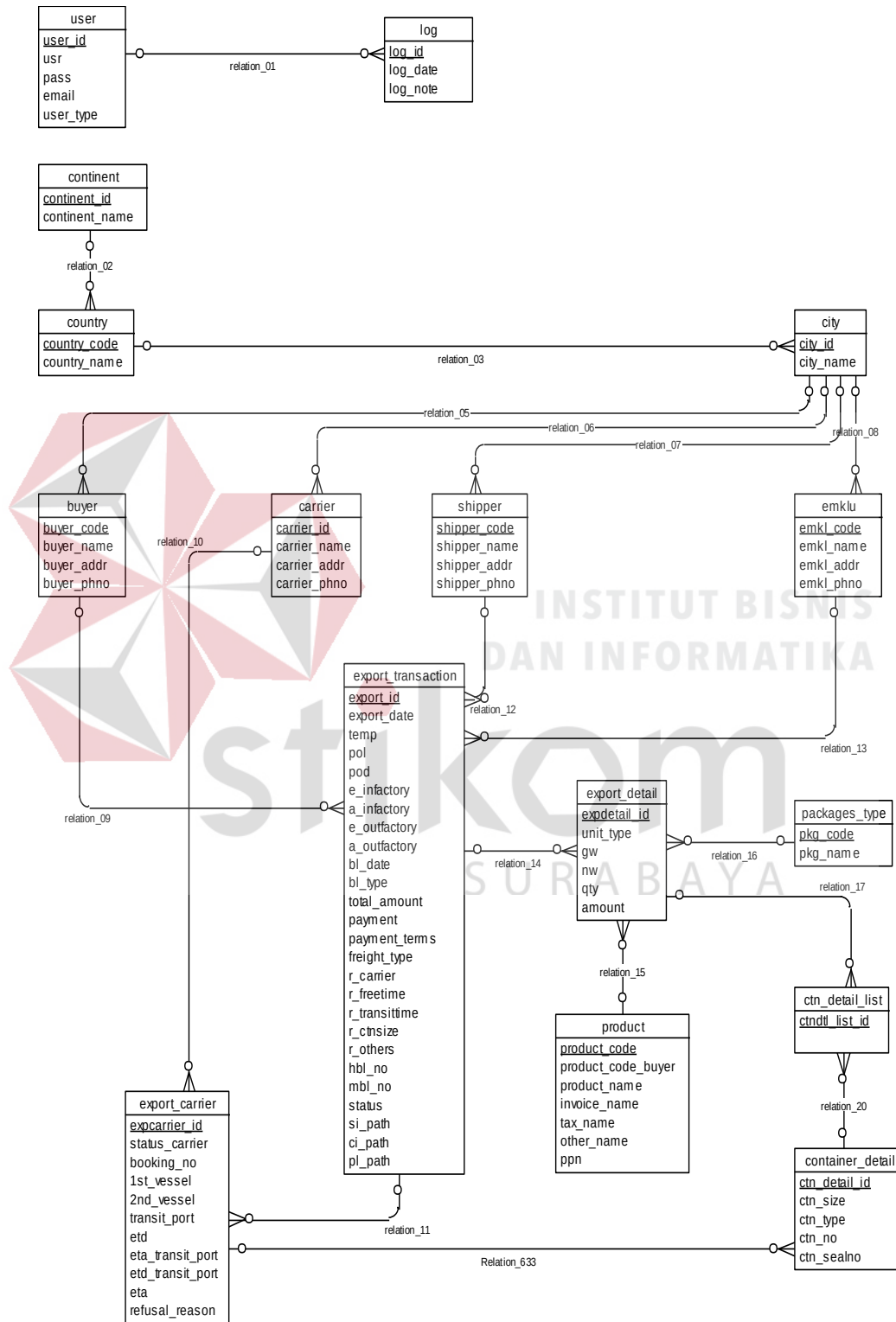
Gambar 0.32 Conceptual data model (CDM)
