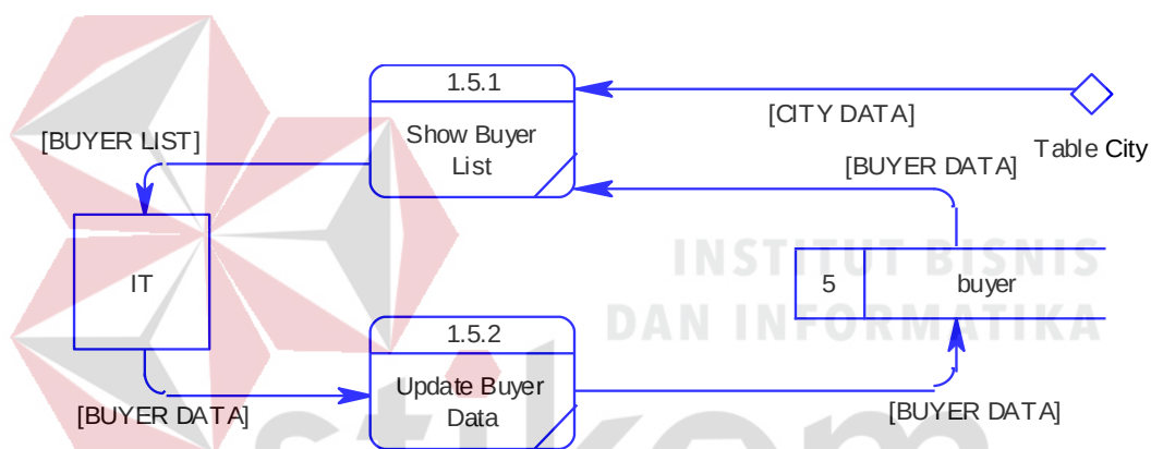
Gambar 0.28 Data flow diagram level 2 manage master data buyer
