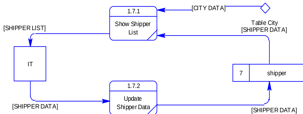
Gambar 0.30 Data flow diagram level 2 manage master data shipper
