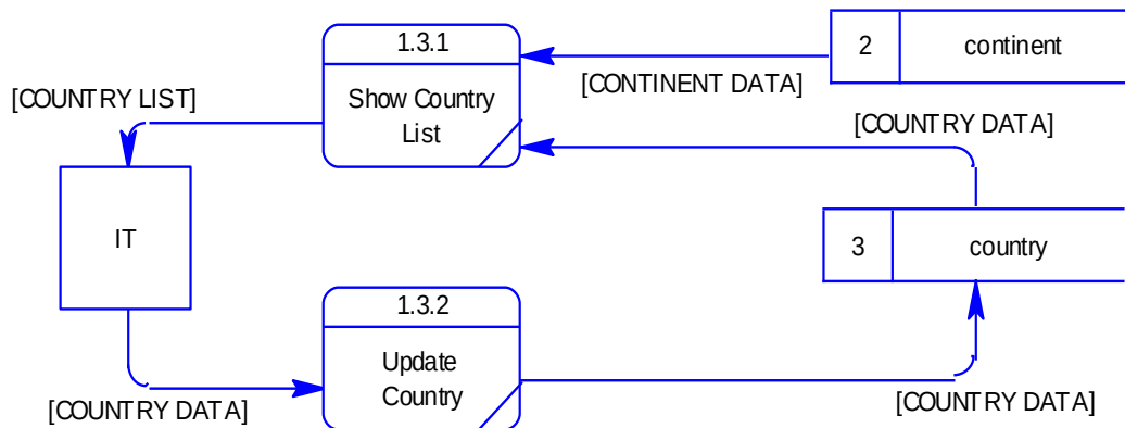
Gambar 0.26 Data flow diagram level 2 manage master data country
