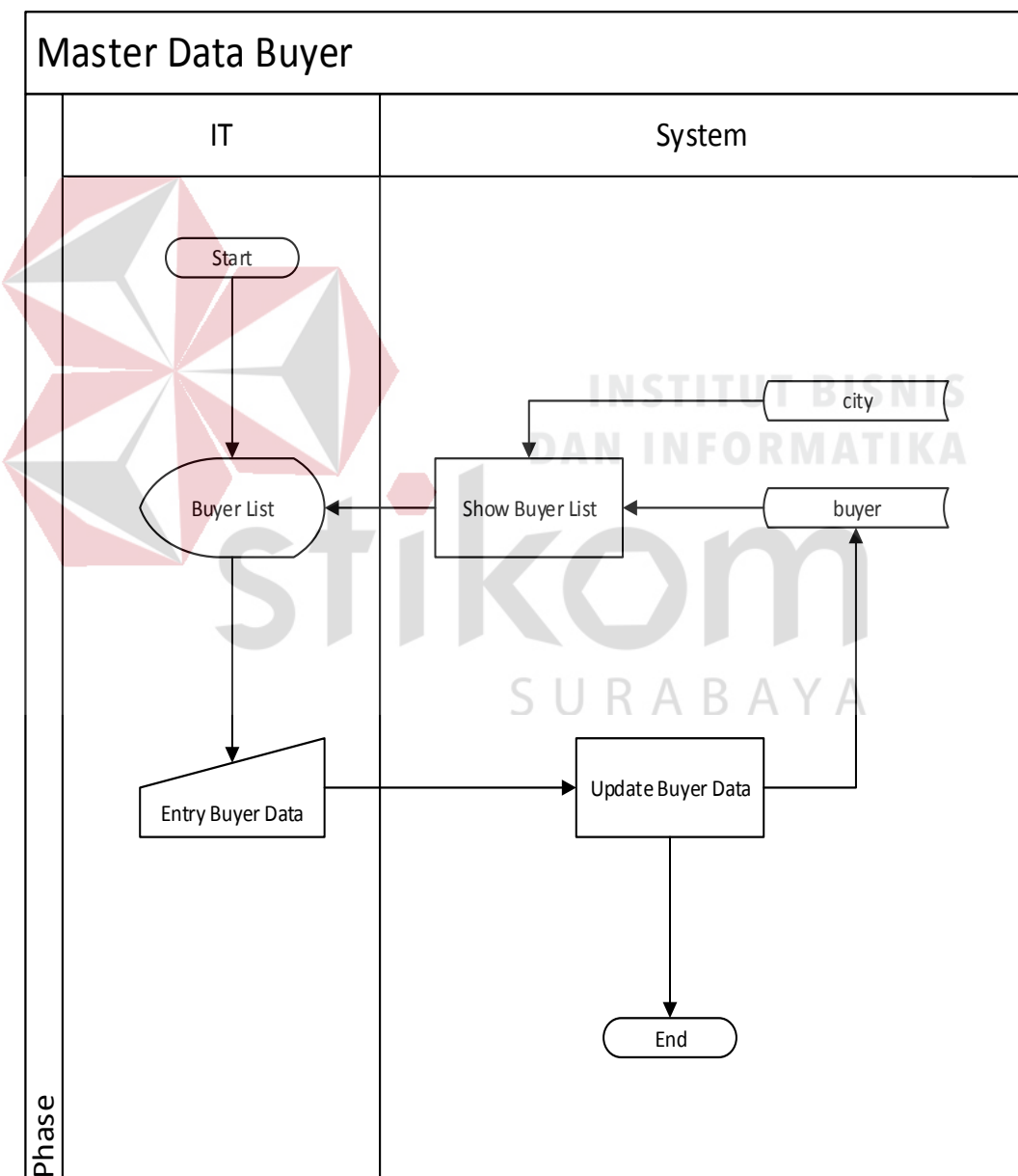
Gambar 0.9 System flow data master buyer
