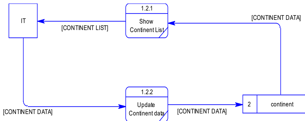
Gambar 4.25 Data flow diagram level 2 manage master data continent
