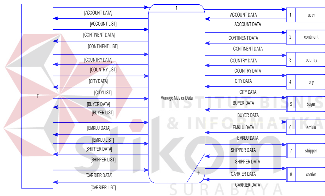
Gambar 4.18 Data flow diagram level 0 manage data master
