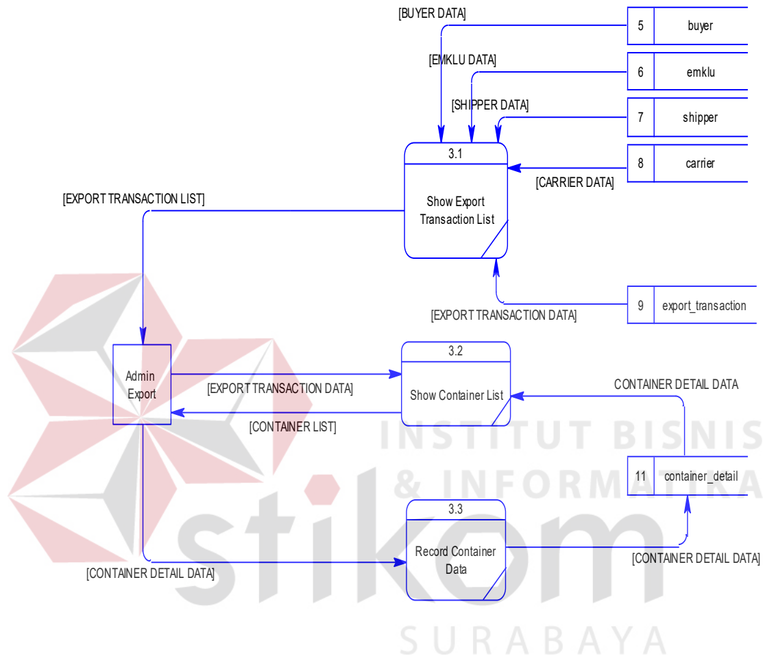
Gambar 4.22 Data flow diagram level 1 set container
