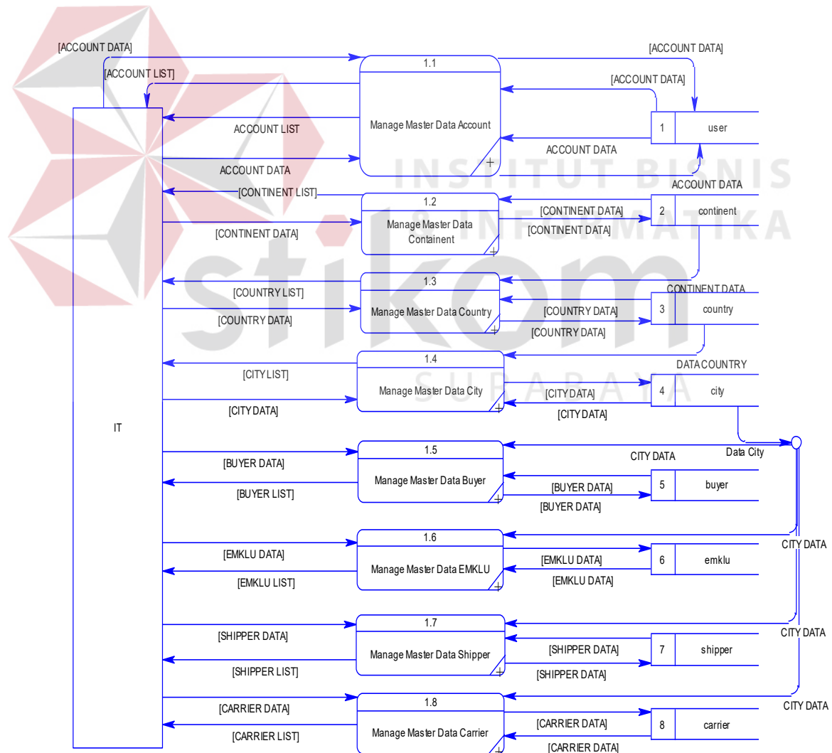
Gambar 4.20 Data flow diagram level 1 manage master data
