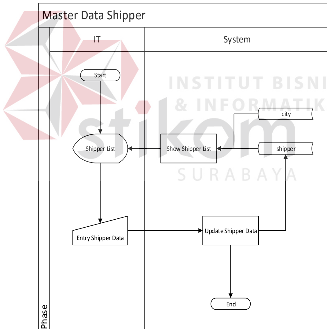
Gambar 4.11 System flow data master shipper
