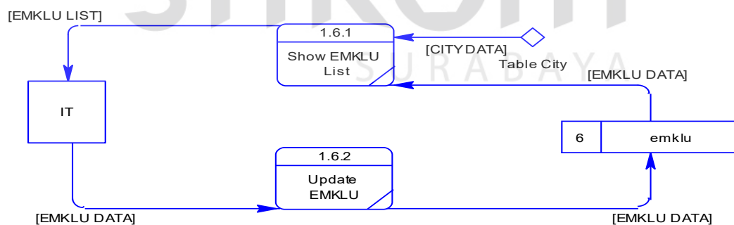
Gambar 4.29 Data flow diagram level 2 manage master data EMK
