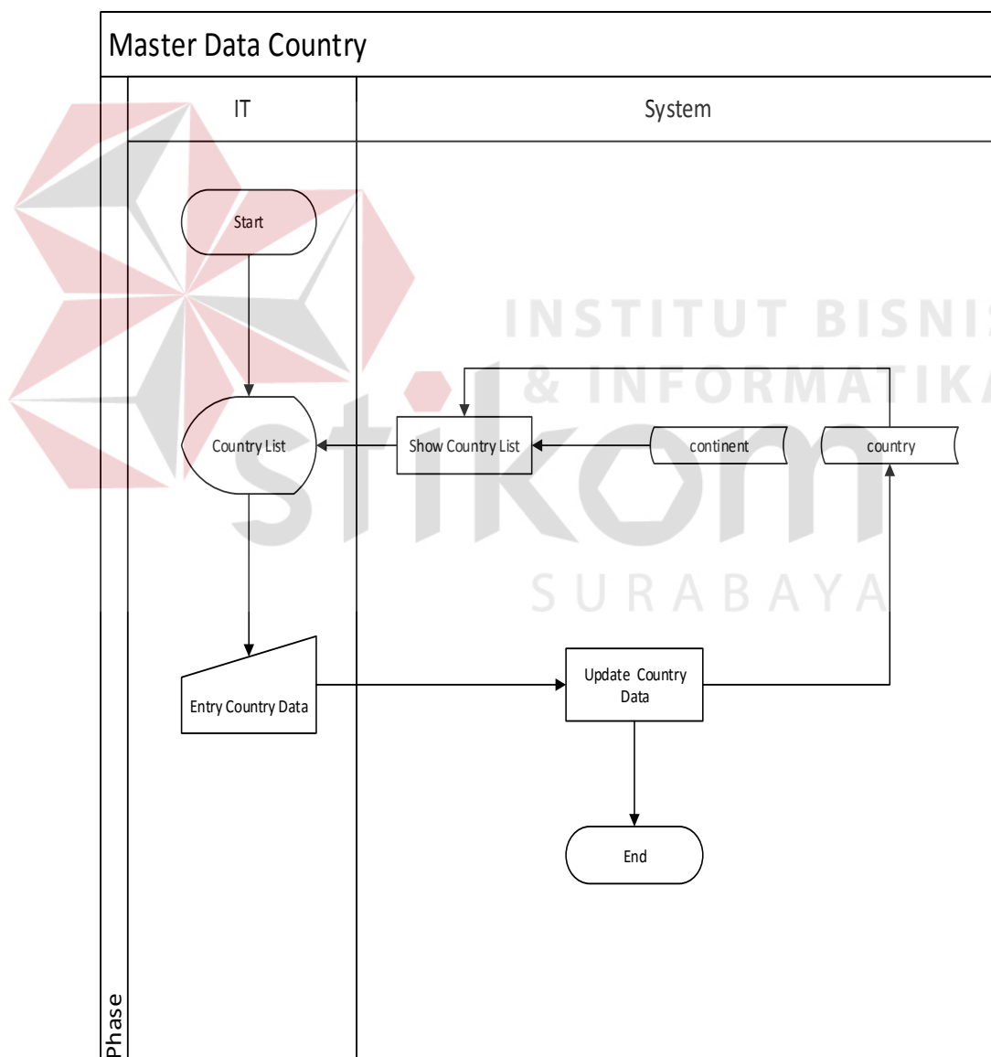
Gambar 4.7 System flow data master country
