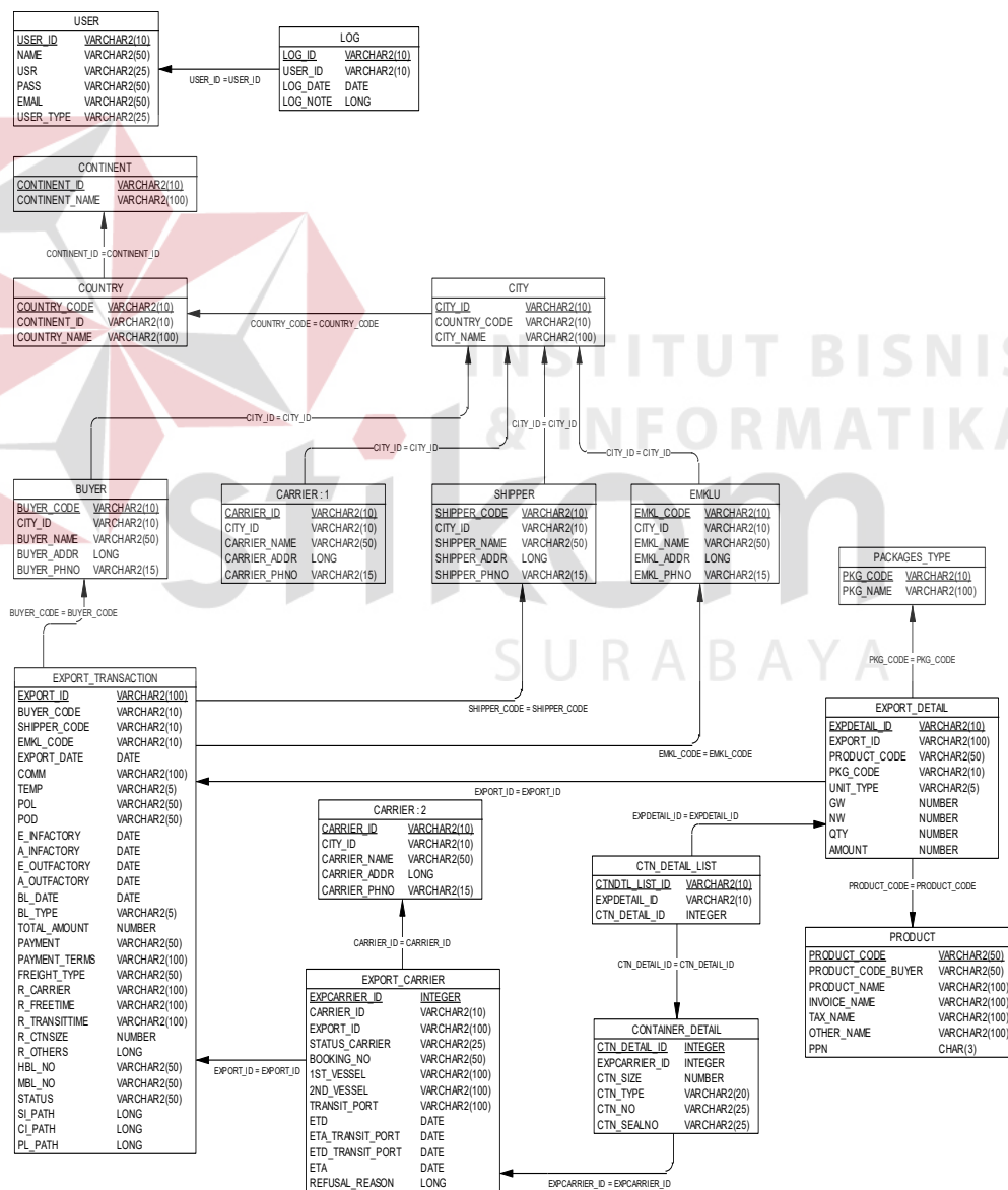
Gambar 4.33 Physical Data Model (PDM)
