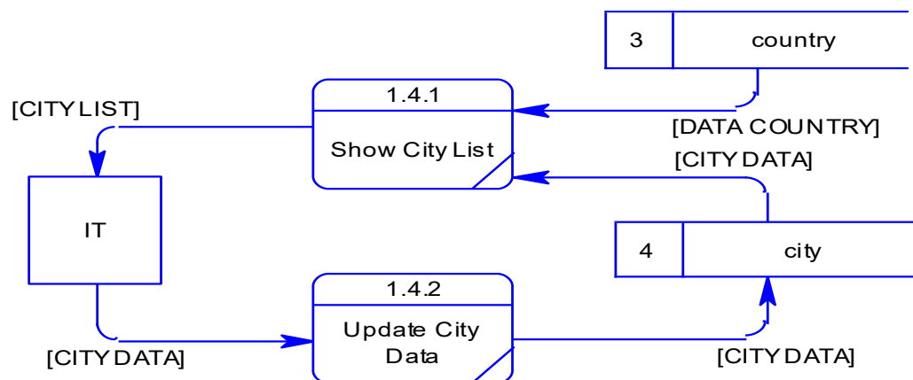
Gambar 4.27 Data flow diagram level 2 manage master data city
