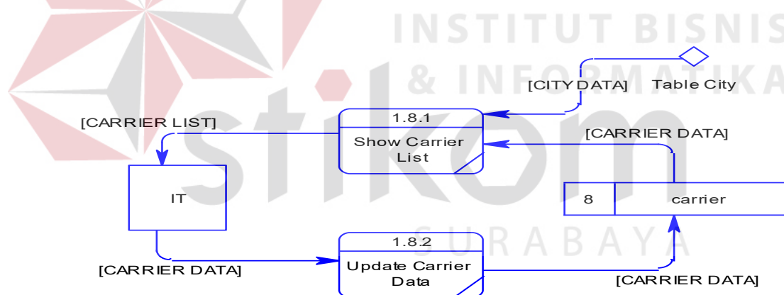
Gambar 4.31 Data flow diagram level 2 manage master data carrier
