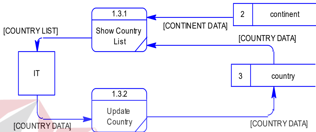
Gambar 4.26 Data flow diagram level 2 manage master data country
