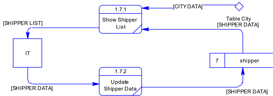
Gambar 4.30 Data flow diagram level 2 manage master data shipper
