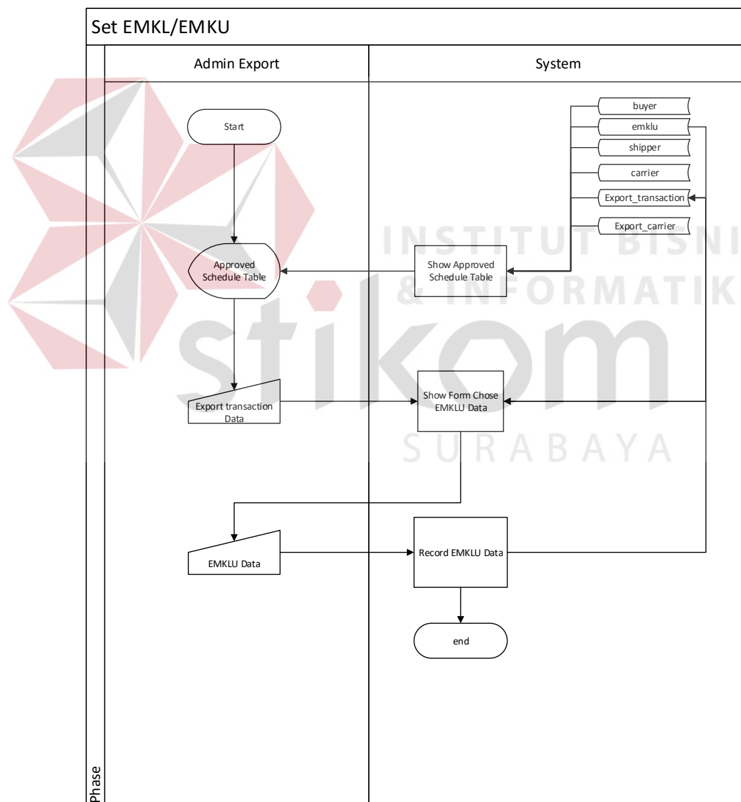
Gambar 4.13 System Flow set EMKL-EMKU
