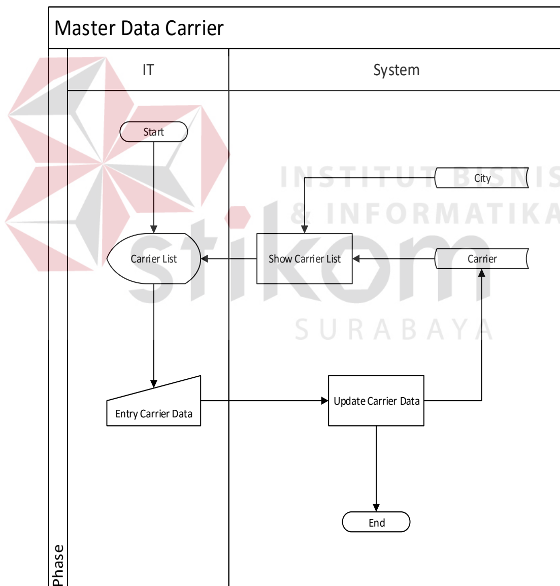
Gambar 4.12 System flow data master carrier
