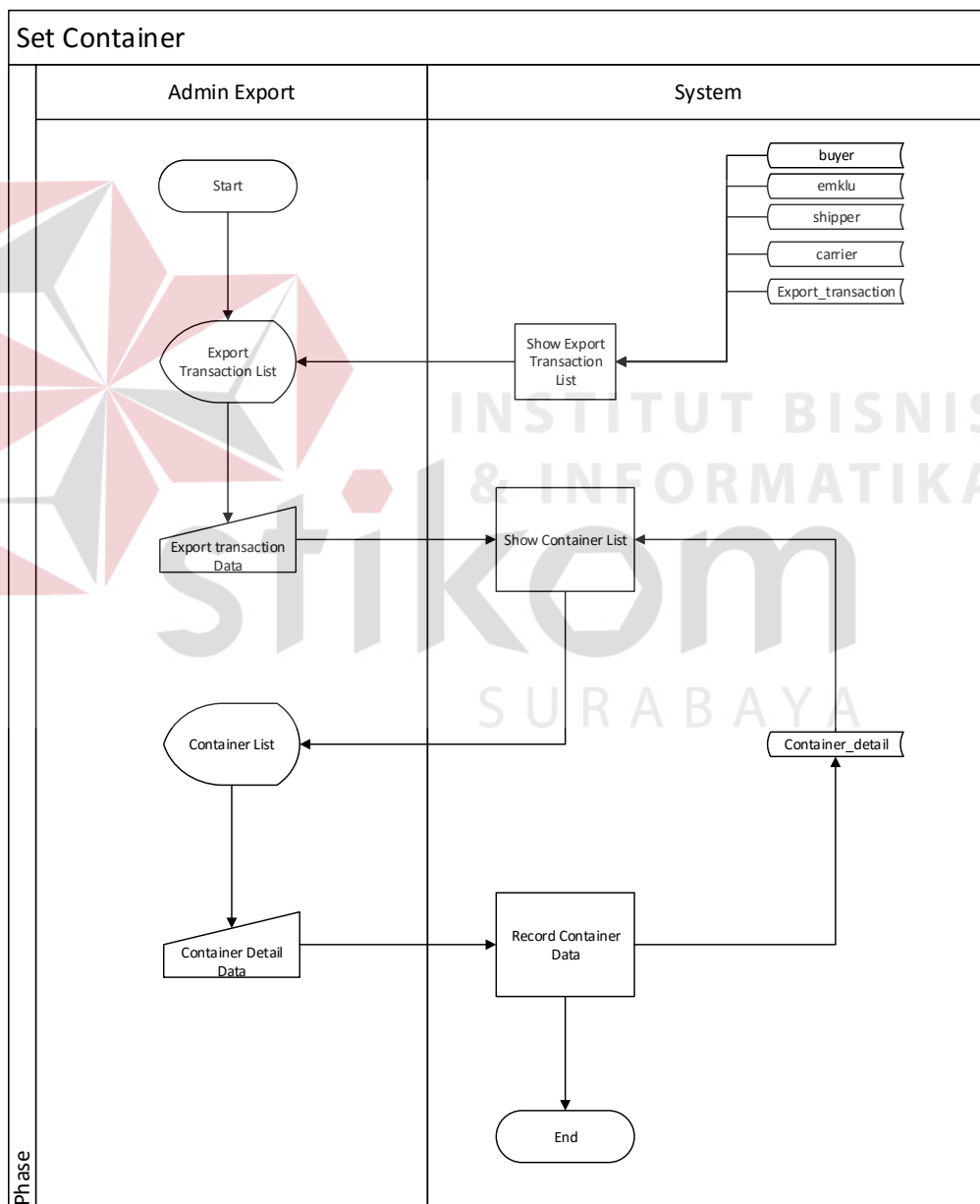
Gambar 4.14 System flow set container
