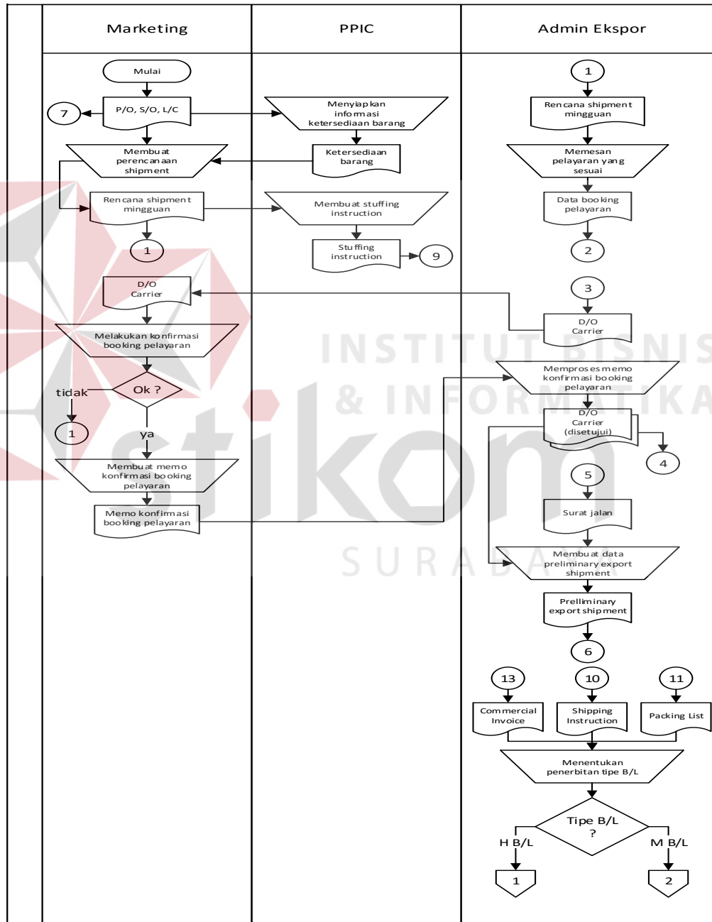
Gambar 4.1 Document flow export
