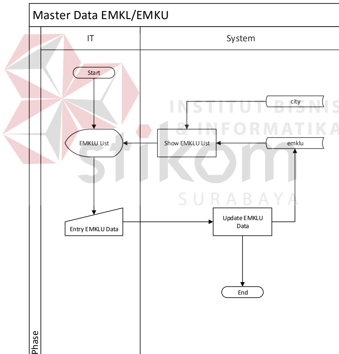
Gambar 4.10 System flow data master EMKLU
