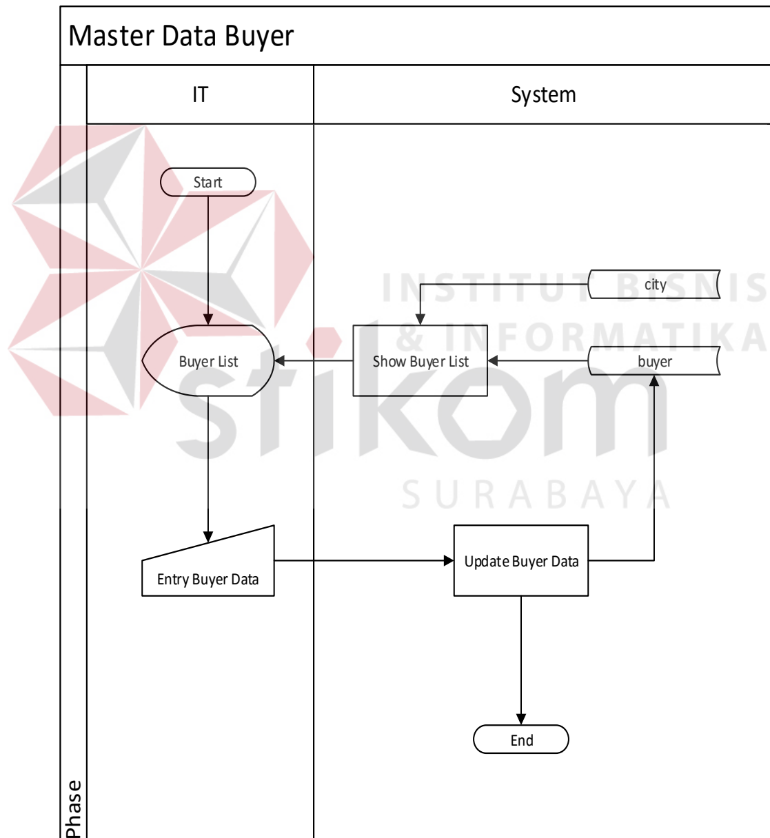
Gambar 4.9 System flow data master buyer
