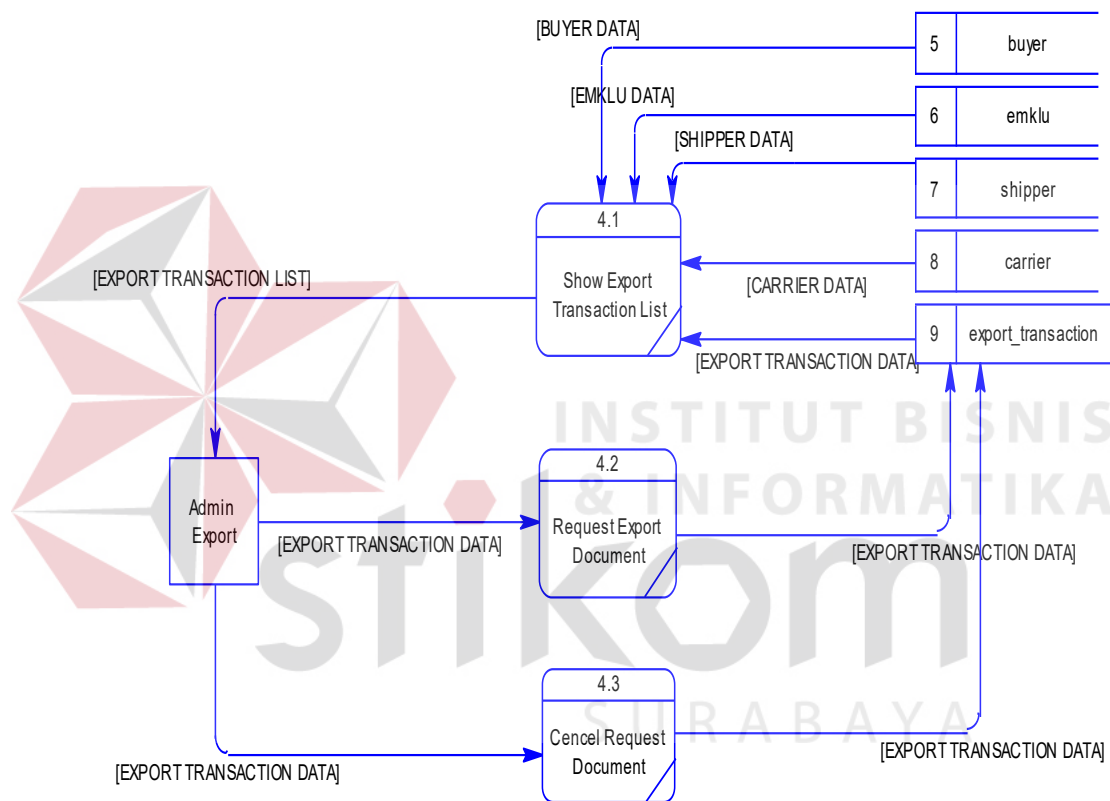
Gambar 4.23 Data flow diagram level 1 document request
