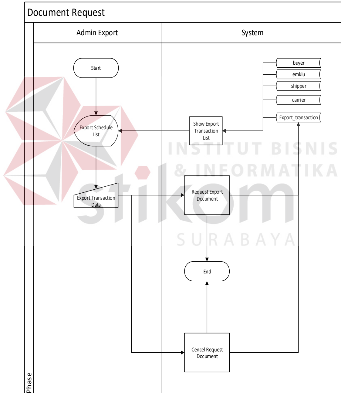
Gambar 4.15 System flow document request
