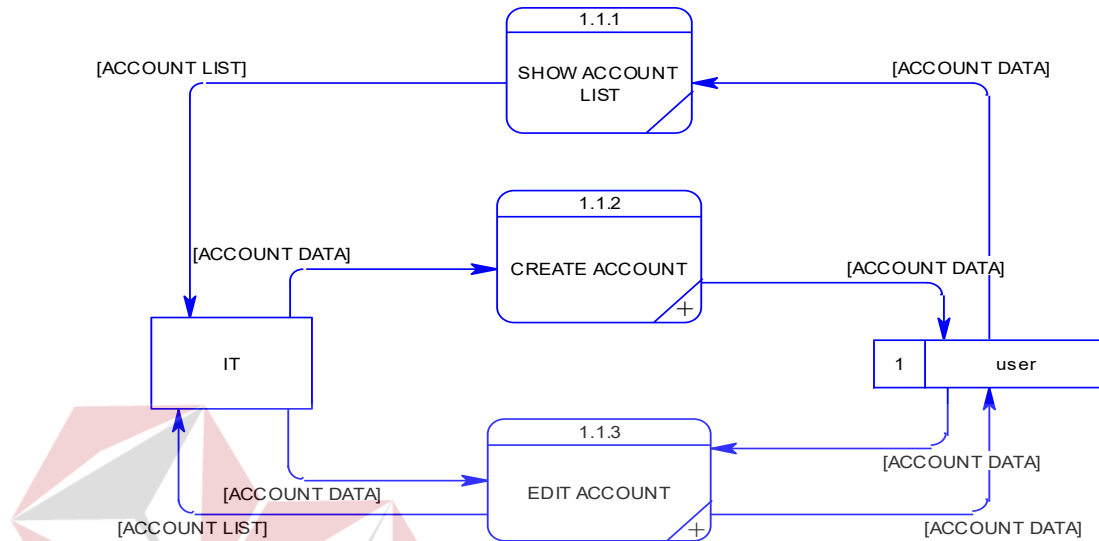
Gambar 4.24 Data flow diagram level 2 manage master data account
