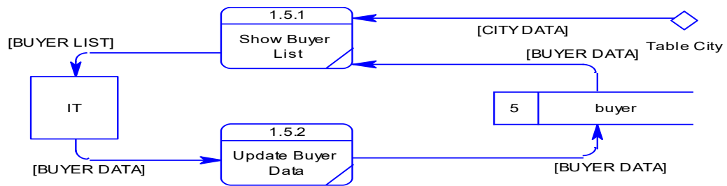
Gambar 4.28 Data flow diagram level 2 manage master data buyer
