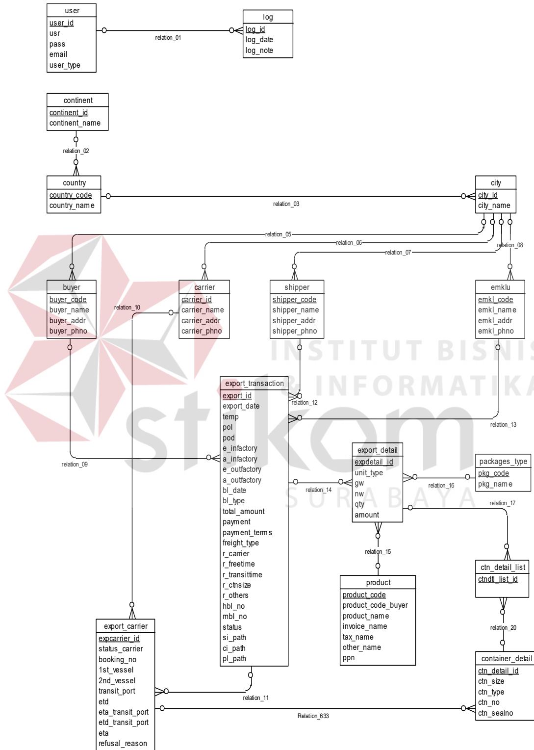
Gambar 4.32 Conceptual data model (CDM)
