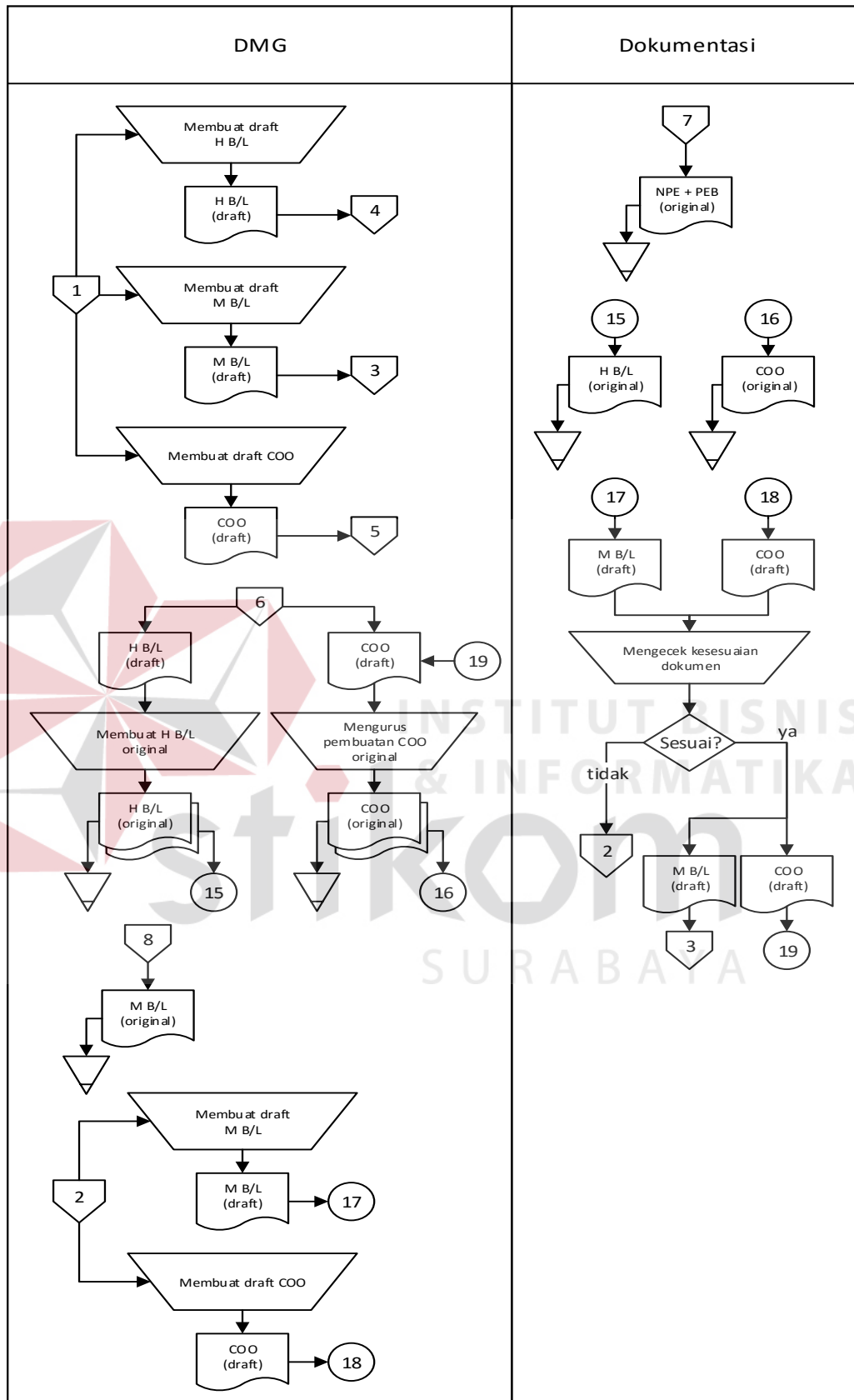
Gambar 4.3 Document flow export
