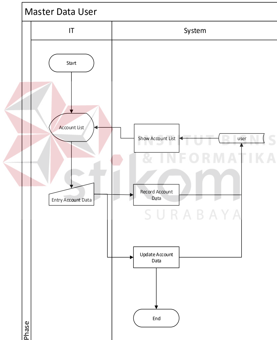
Gambar 4.5 System flow data master user
