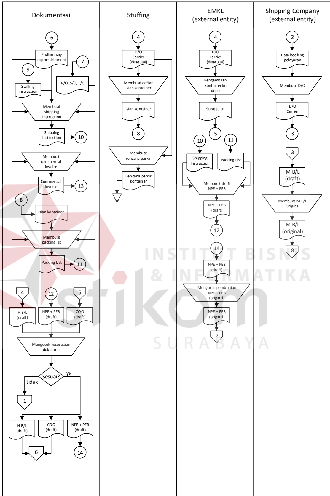
Gambar 4.2 Document flow export
