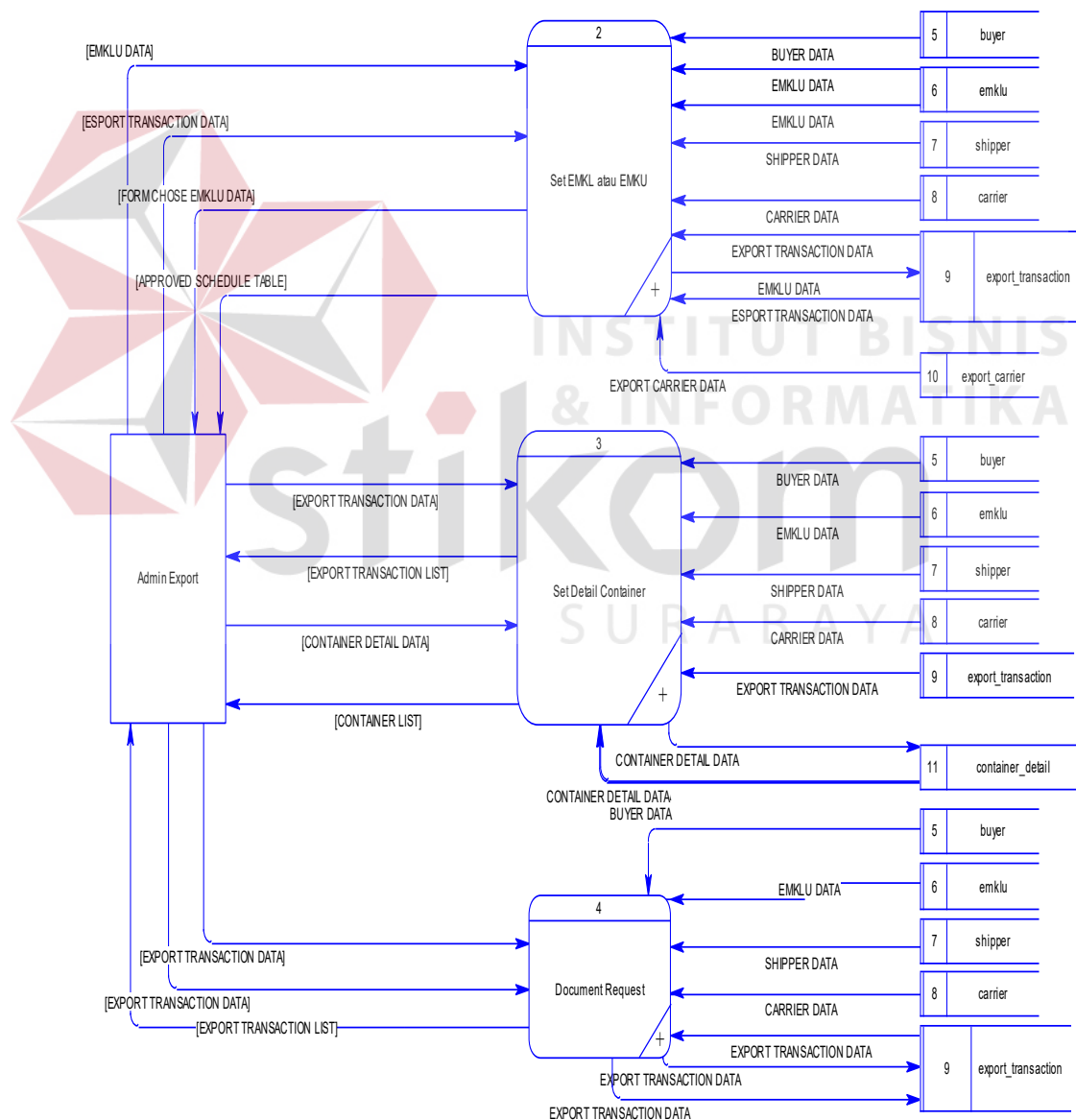
Gambar 4.19 Data flow diagram level 0 transaction
