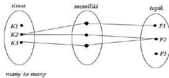
Gambar 3.14 Tipe relasi many to many
