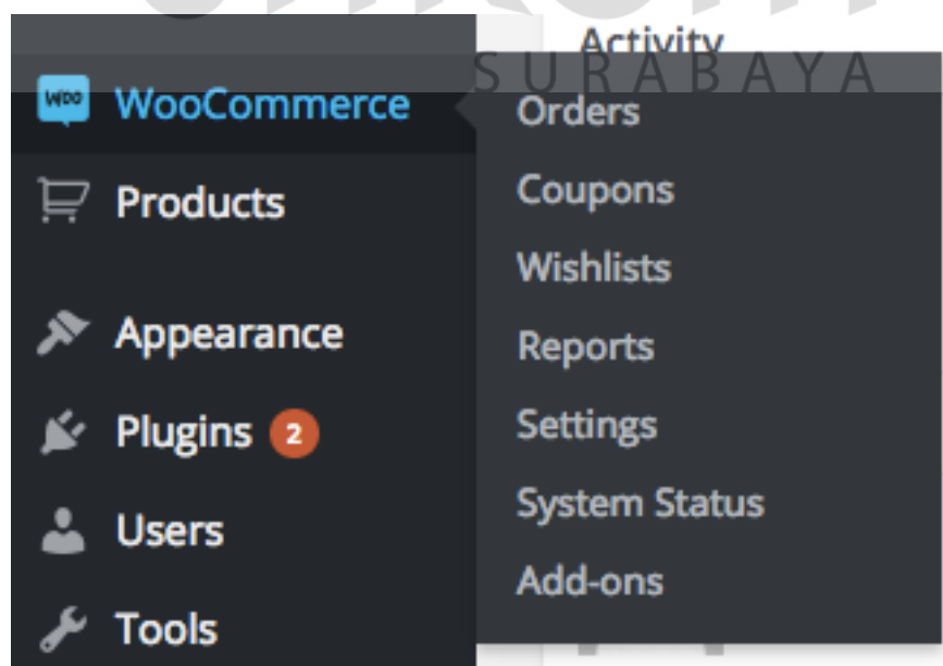
Gambar 4.32 menu orders
