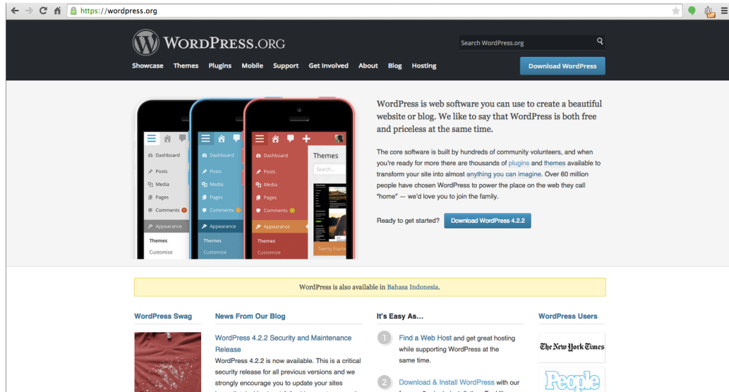
Gambar 4.3 Homepage www.wordpress.org
