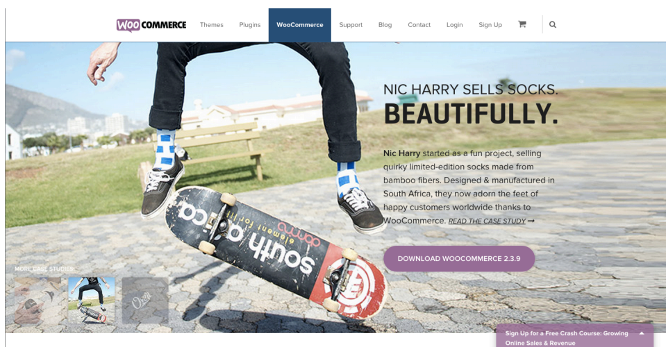
Gambar 4.10 Website wocommerce
