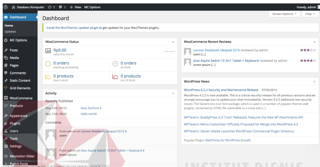
Gambar 4.15 Halaman Dashboard
