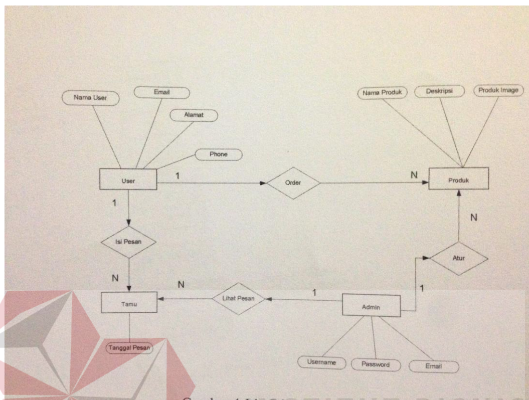
Gambar 4.14 : Diagram E-R
