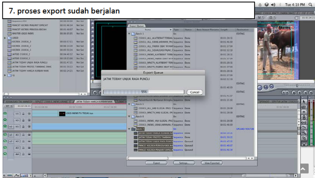
Gambar 4.7 proses render
