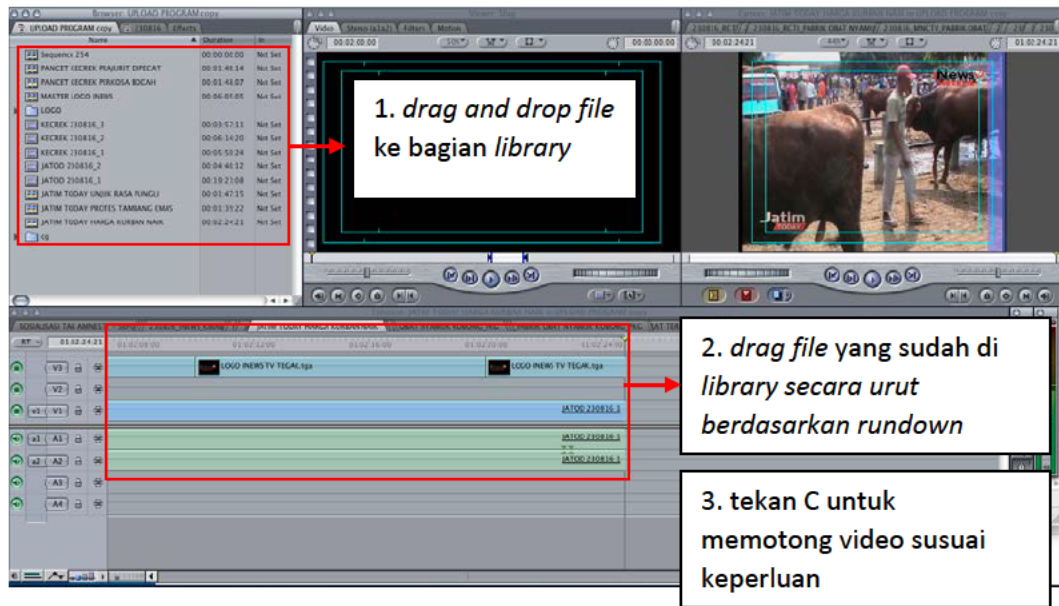
Gambar 4.5 proses editing
