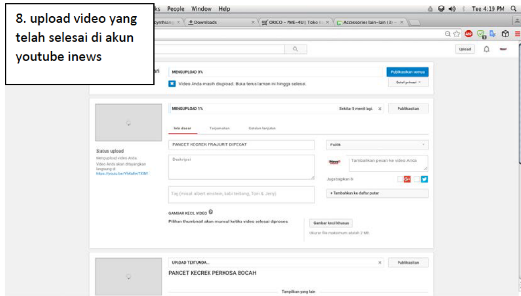
Gambar 4.9 proses upload
