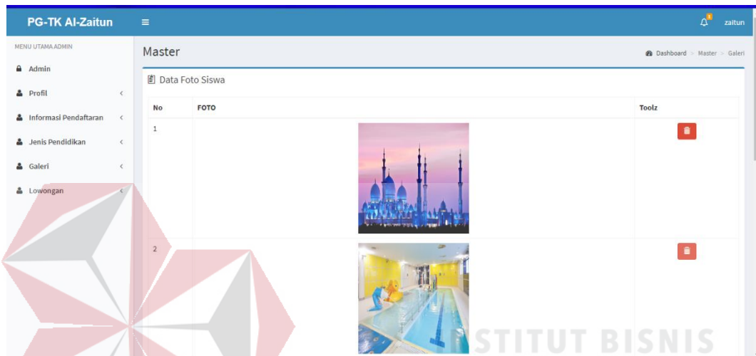
Gambar 1. 18 Admin Galeri
