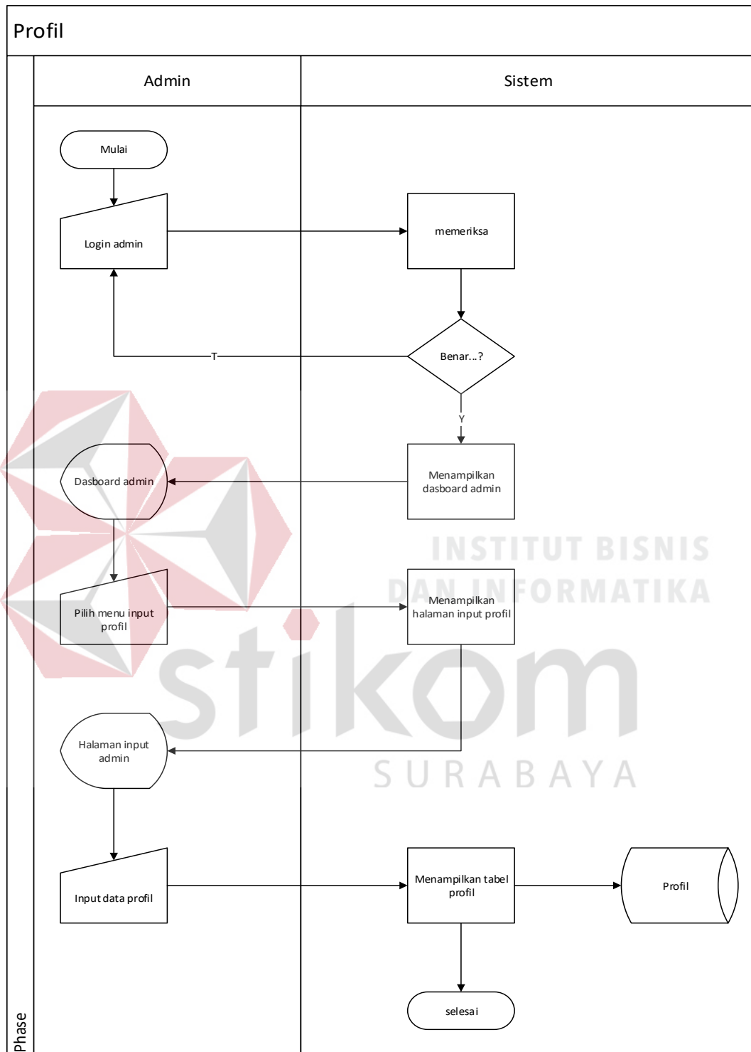
Gambar 1. 2 Sistem Flow Maintenance Data Profil
