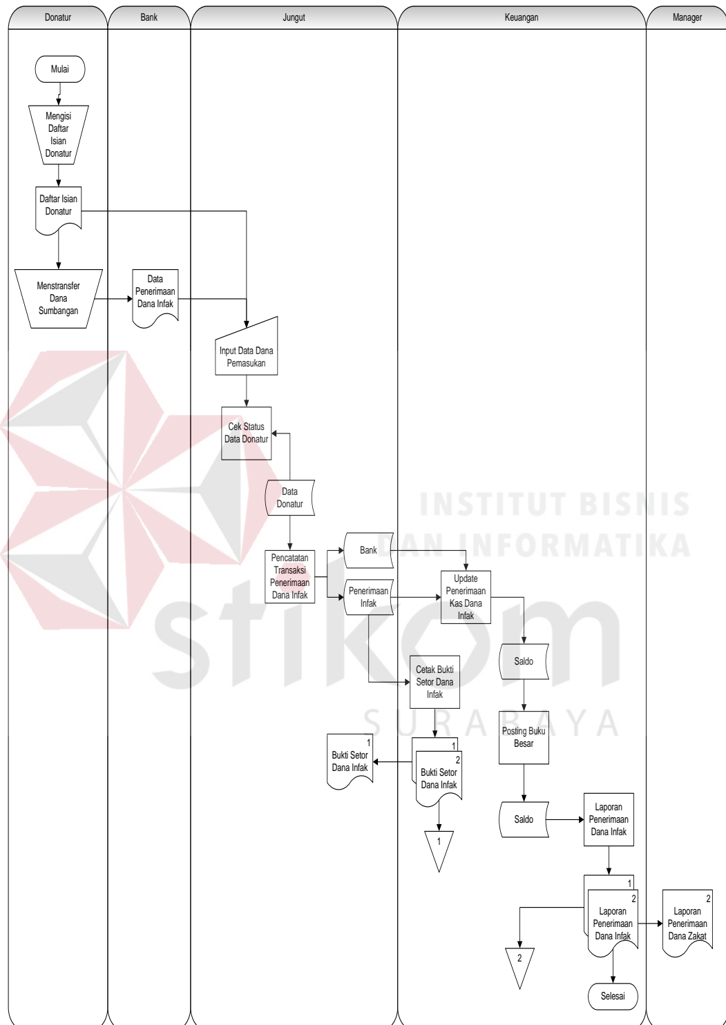
System Flow Penerimaan Dana Infak/Sedekah
