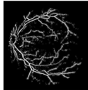
Gambar 5. Citra Biner
