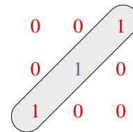
Gambar 6. Structure Element
