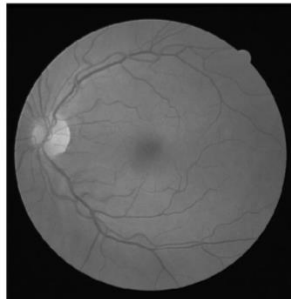
Gambar 3. Citra Grayscale
