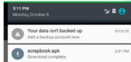
Gambar 1. Proses download
