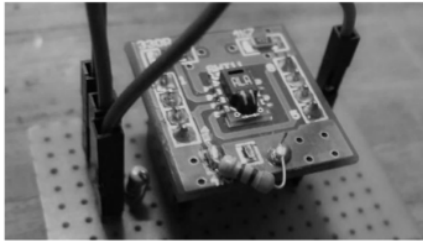
Gbr. 4 Sensor SHT 11.
