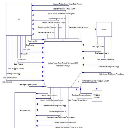
Gambar 3. Context Diagram
