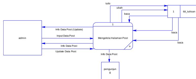
Gambar 4.13 DFD Level 1 Mengelola Halaman Post Event
