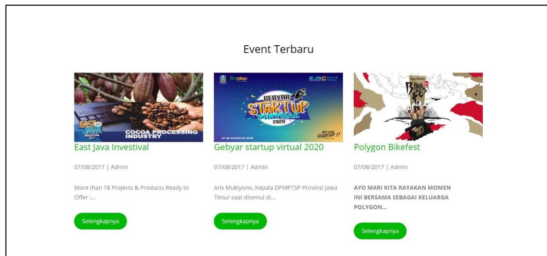
Gambar 4.49 Halaman Event
