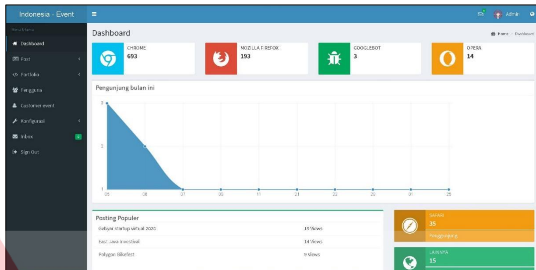
Gambar 4.29 Halaman Dashboard
