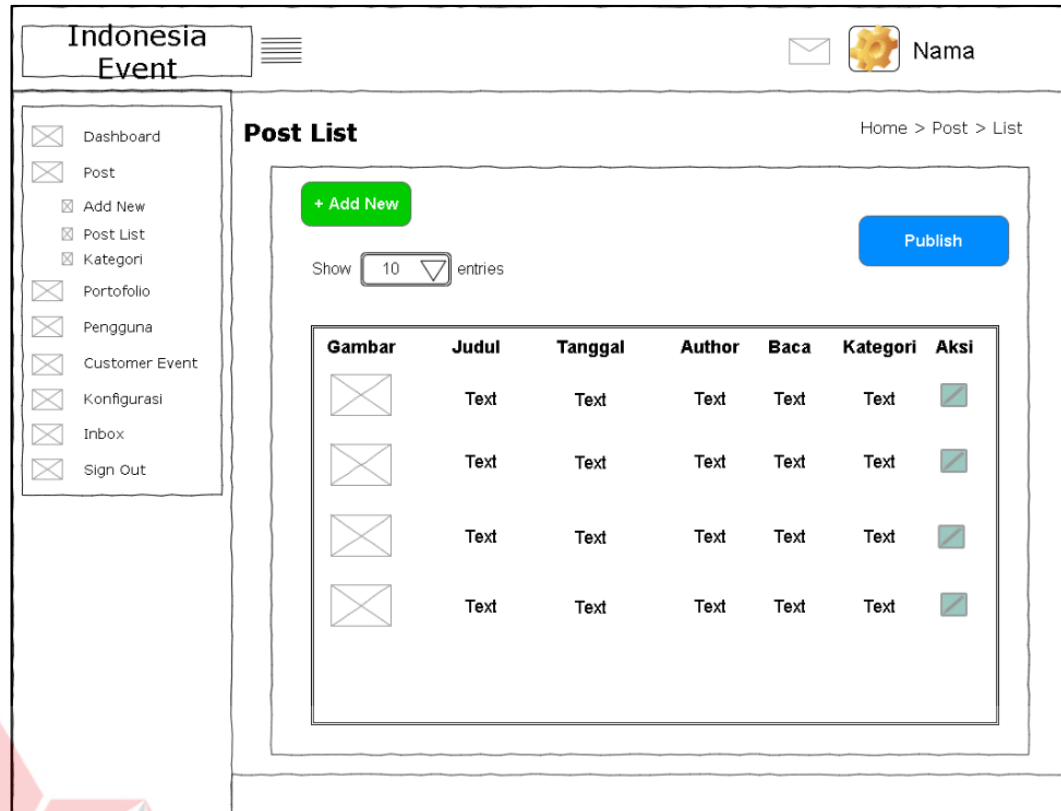
Gambar 4.27 Halaman Post List Event
