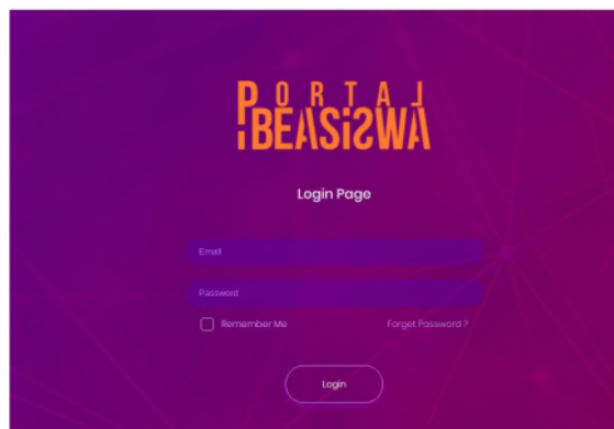
Gambar 2 Login Form
