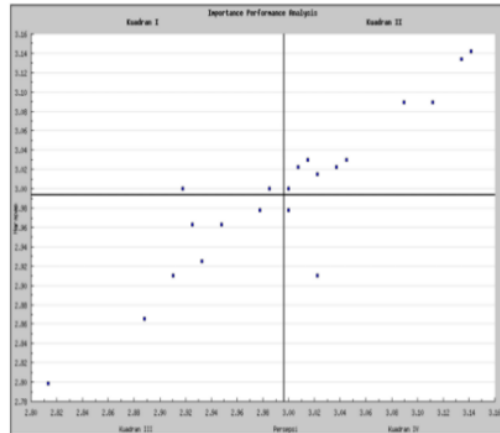
Gambar 9. Analisis Kuadran
