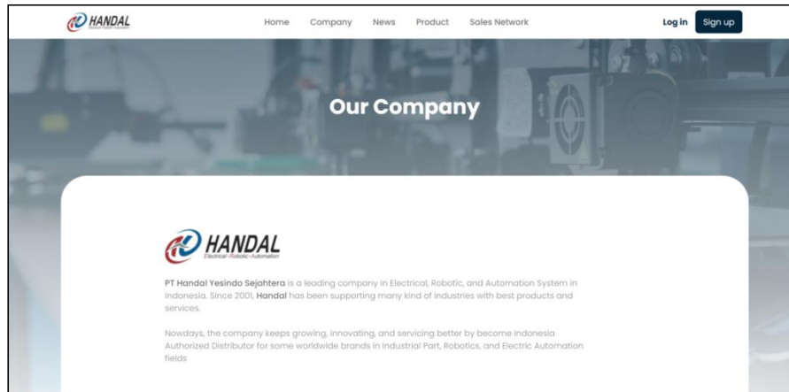
Gambar 3.9 Halaman Company
