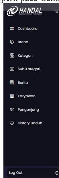
Gambar 3.4 Dashboard Admin
