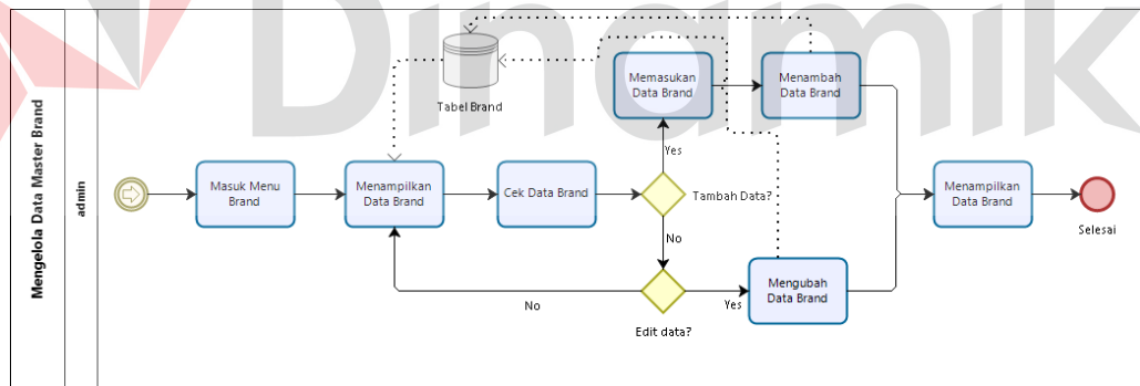
Gambar 1.6 Mengelola Data Master Brand
