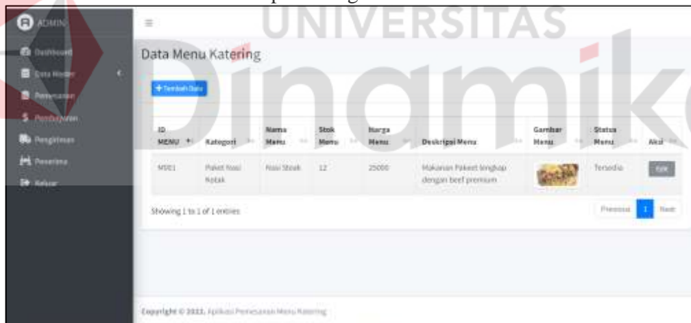
Gambar 3.6 Halaman Data Master Menu
