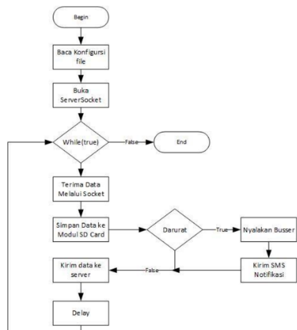
Gambar 5. Flowchart IOT Master Controller
