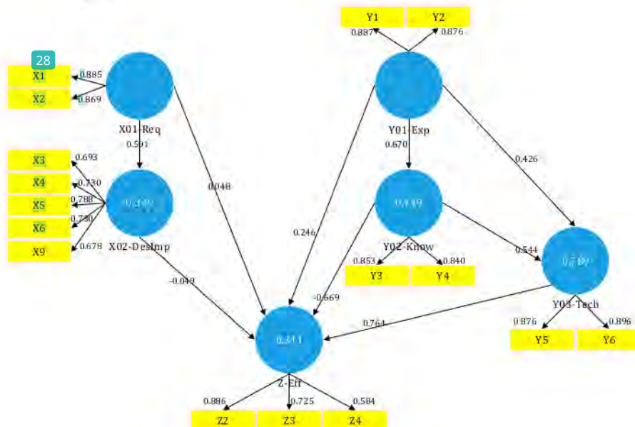
Figure 3. Confirmed Path Coefficient Model
