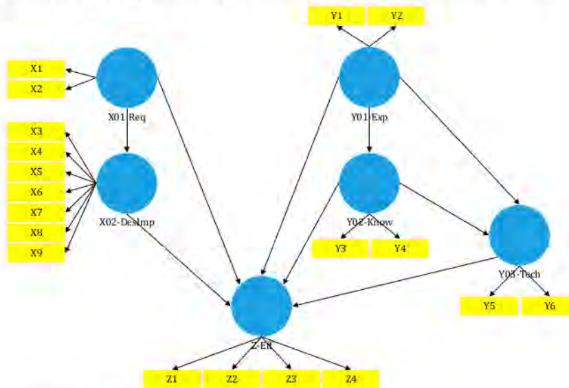
Figure 2. Preliminary Path Coefficient Model
