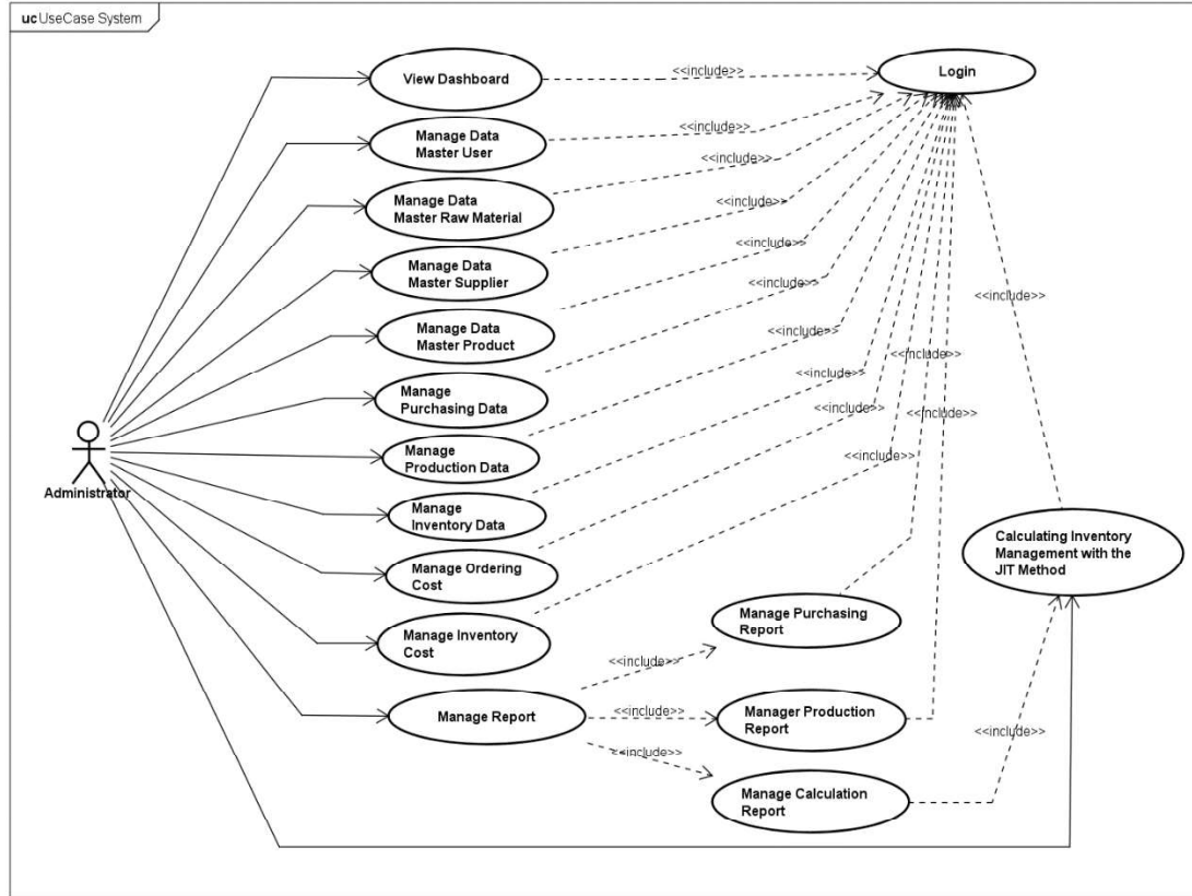
Figure 2. Use Case System
