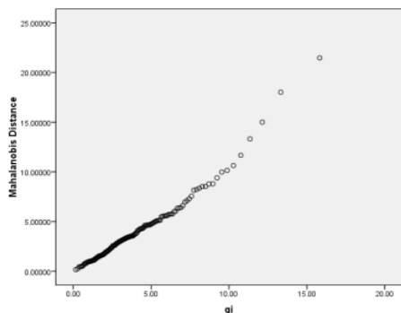
Gambar 1 Scatter-Plot Hasil Uji Normalitas Data
