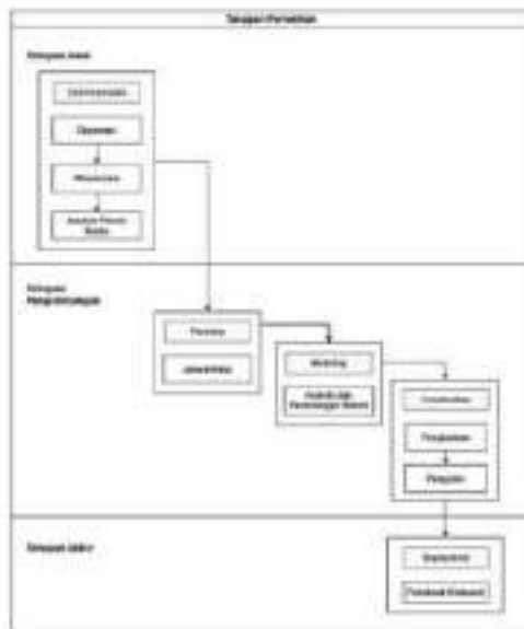
Gambar 1. Model Waterfall
