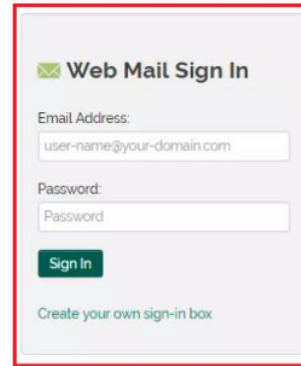
Gambar 6. Phishing WebPage
