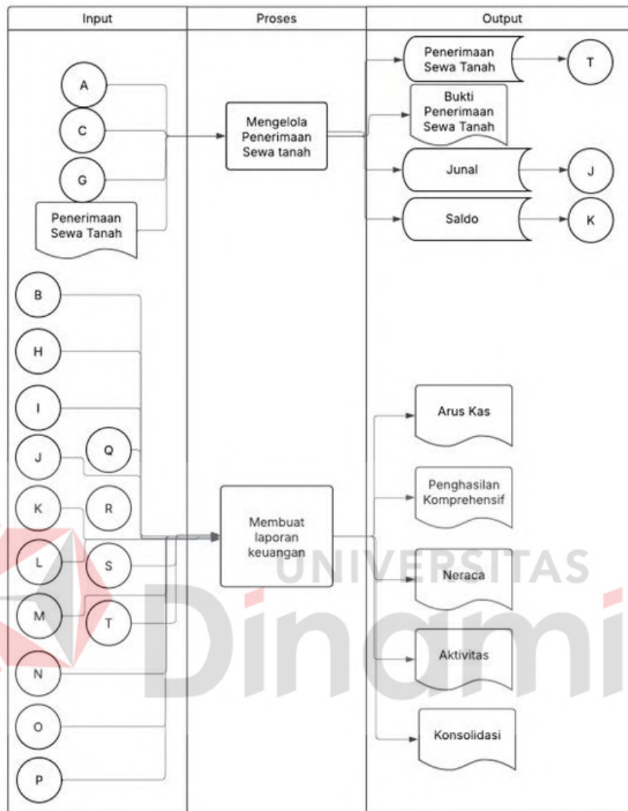
Gambar 2. 12 Diagram IPO 4
