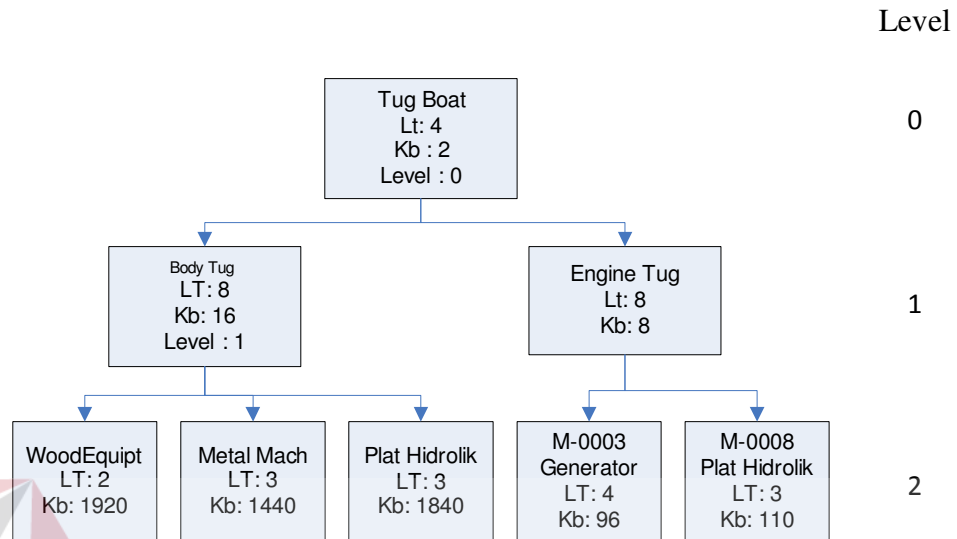
Gambar 4.20. Diagram Tree Manual Bill of Material
